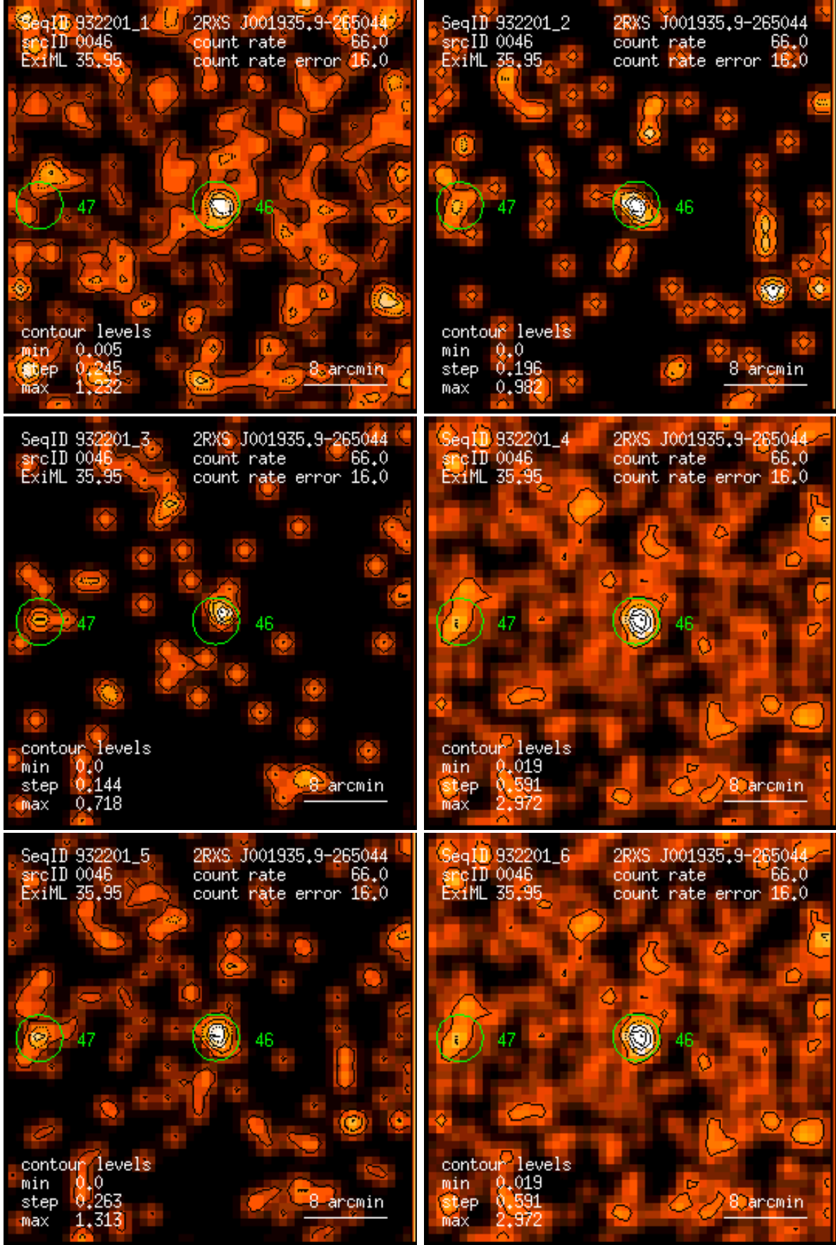
Figure 46: RASS 932201: detection 0046: band rate images, Gaussian filter: (1) PSPC channels 11 – 41, (2) 52 – 90, (3) 91 – 201, (4) 11 – 235, (5) 52 – 201, (6) 11 – 201. Broad band rates in counts/ks. Band rate contour levels in counts/ks/arcmin 2 .
