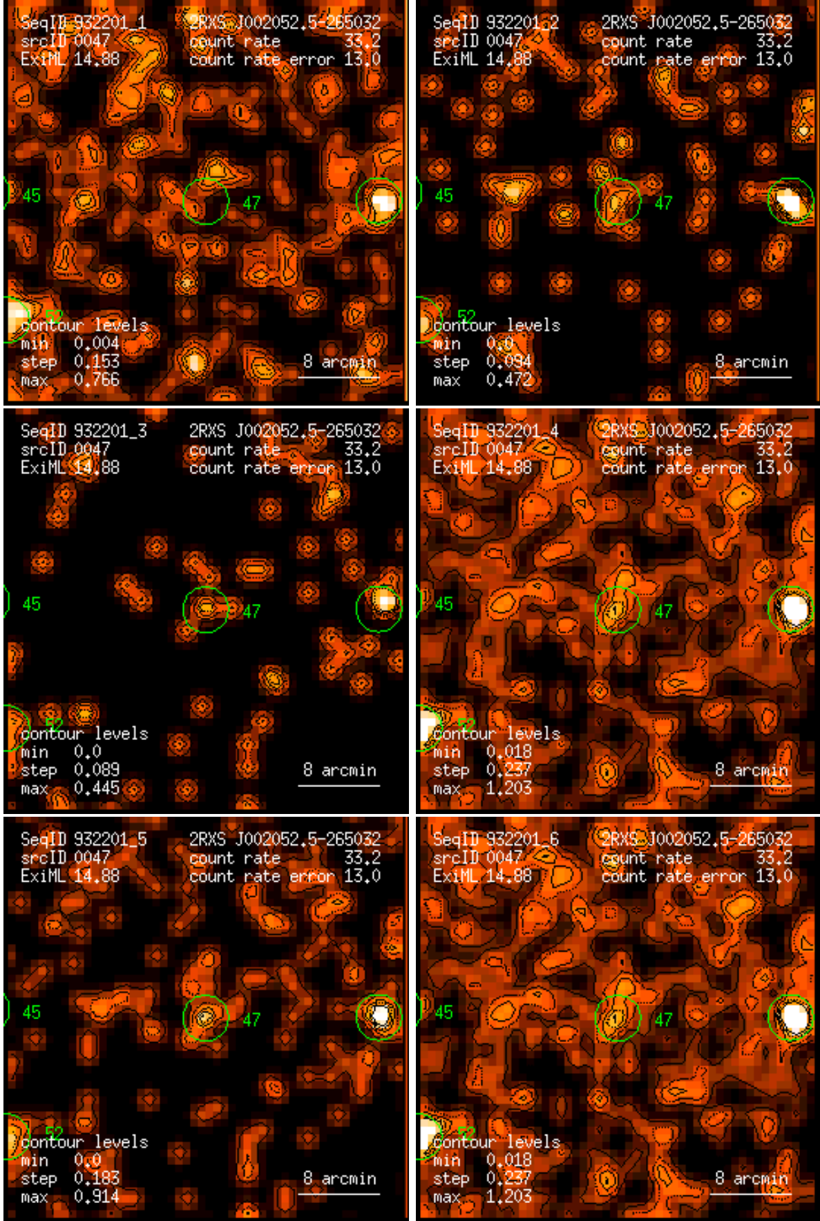
Figure 47: RASS 932201: detection 0047: band rate images, Gaussian filter: (1) PSPC channels 11 – 41, (2) 52 – 90, (3) 91 – 201, (4) 11 – 235, (5) 52 – 201, (6) 11 – 201. Broad band rates in counts/ks. Band rate contour levels in counts/ks/arcmin 2 .
