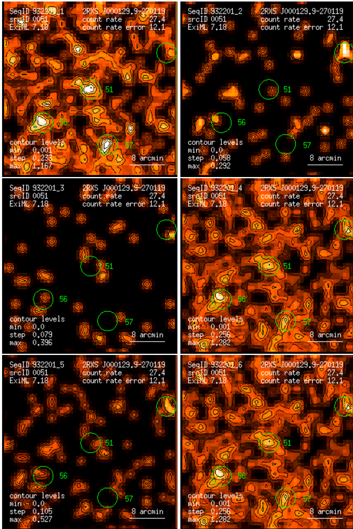
Figure 51: RASS 932201: detection 0051: band rate images, Gaussian filter: (1) PSPC channels 11 – 41, (2) 52 – 90, (3) 91 – 201, (4) 11 – 235, (5) 52 – 201, (6) 11 – 201. Broad band rates in counts/ks. Band rate contour levels in counts/ks/arcmin 2 .
