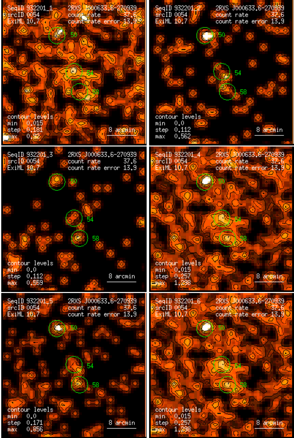
Figure 54: RASS 932201: detection 0054: band rate images, Gaussian filter: (1) PSPC channels 11 – 41, (2) 52 – 90, (3) 91 – 201, (4) 11 – 235, (5) 52 – 201, (6) 11 – 201. Broad band rates in counts/ks. Band rate contour levels in counts/ks/arcmin 2 .
