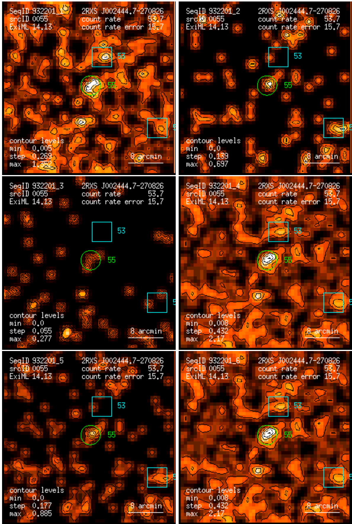
Figure 55: RASS 932201: detection 0055: band rate images, Gaussian filter: (1) PSPC channels 11 – 41, (2) 52 – 90, (3) 91 – 201, (4) 11 – 235, (5) 52 – 201, (6) 11 – 201. Broad band rates in counts/ks. Band rate contour levels in counts/ks/arcmin 2 .
