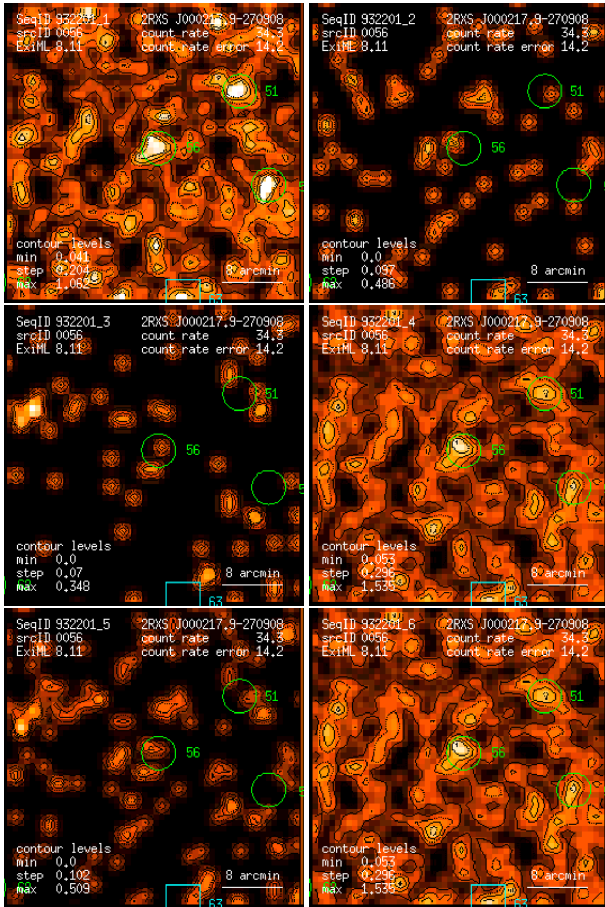
Figure 56: RASS 932201: detection 0056: band rate images, Gaussian filter: (1) PSPC channels 11 – 41, (2) 52 – 90, (3) 91 – 201, (4) 11 – 235, (5) 52 – 201, (6) 11 – 201. Broad band rates in counts/ks. Band rate contour levels in counts/ks/arcmin 2 .
