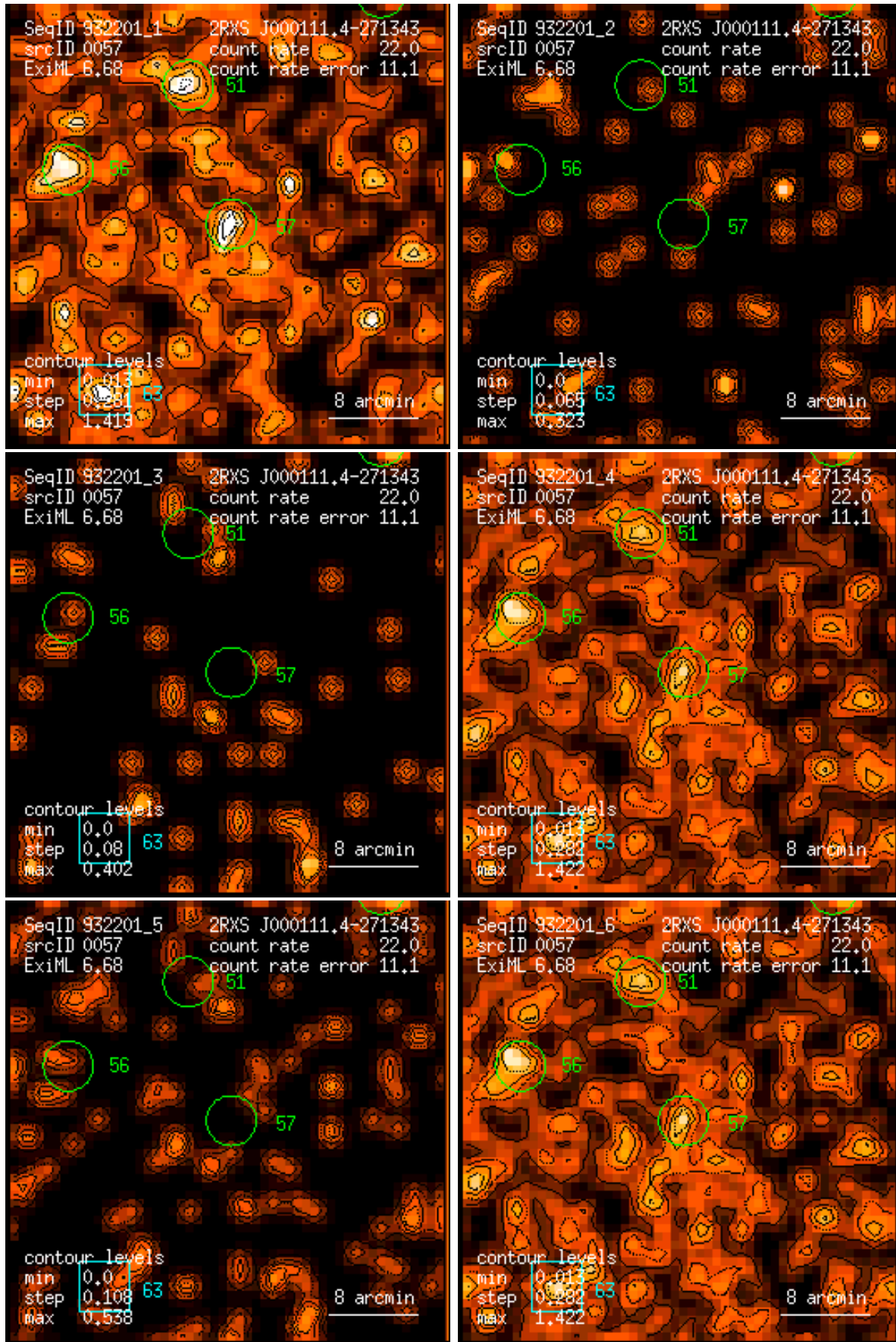
Figure 57: RASS 932201: detection 0057: band rate images, Gaussian filter: (1) PSPC channels 11 – 41, (2) 52 – 90, (3) 91 – 201, (4) 11 – 235, (5) 52 – 201, (6) 11 – 201. Broad band rates in counts/ks. Band rate contour levels in counts/ks/arcmin 2 .
