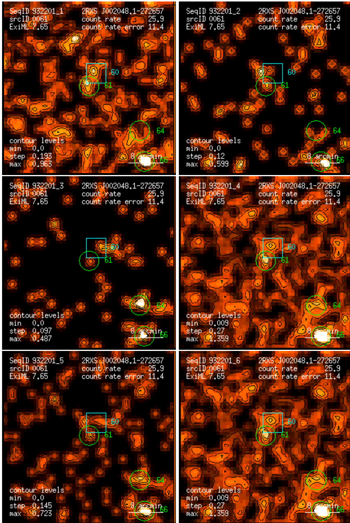
Figure 61: RASS 932201: detection 0061: band rate images, Gaussian filter: (1) PSPC channels 11 – 41, (2) 52 – 90, (3) 91 – 201, (4) 11 – 235, (5) 52 – 201, (6) 11 – 201. Broad band rates in counts/ks. Band rate contour levels in counts/ks/arcmin 2 .
