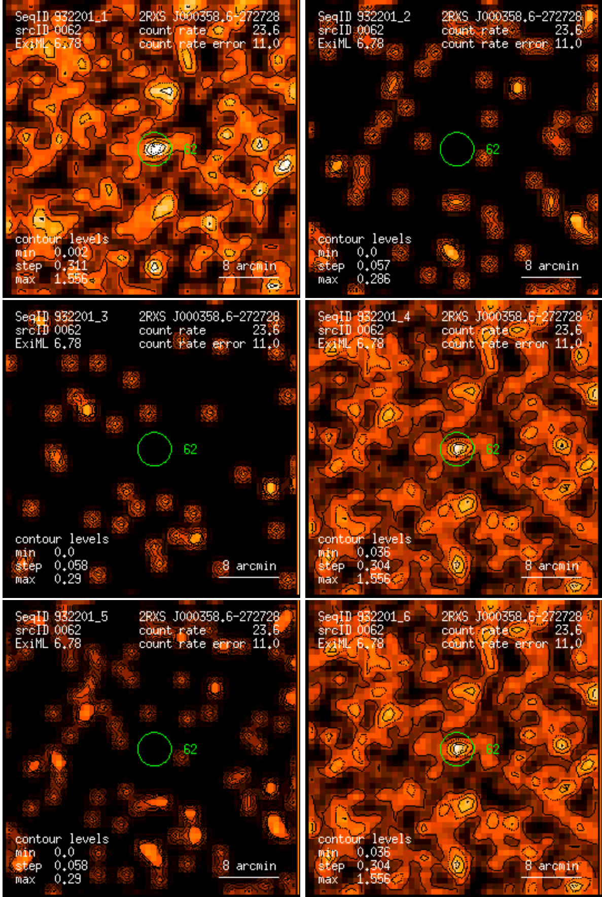
Figure 62: RASS 932201: detection 0062: band rate images, Gaussian filter: (1) PSPC channels 11 – 41, (2) 52 – 90, (3) 91 – 201, (4) 11 – 235, (5) 52 – 201, (6) 11 – 201. Broad band rates in counts/ks. Band rate contour levels in counts/ks/arcmin 2 .
