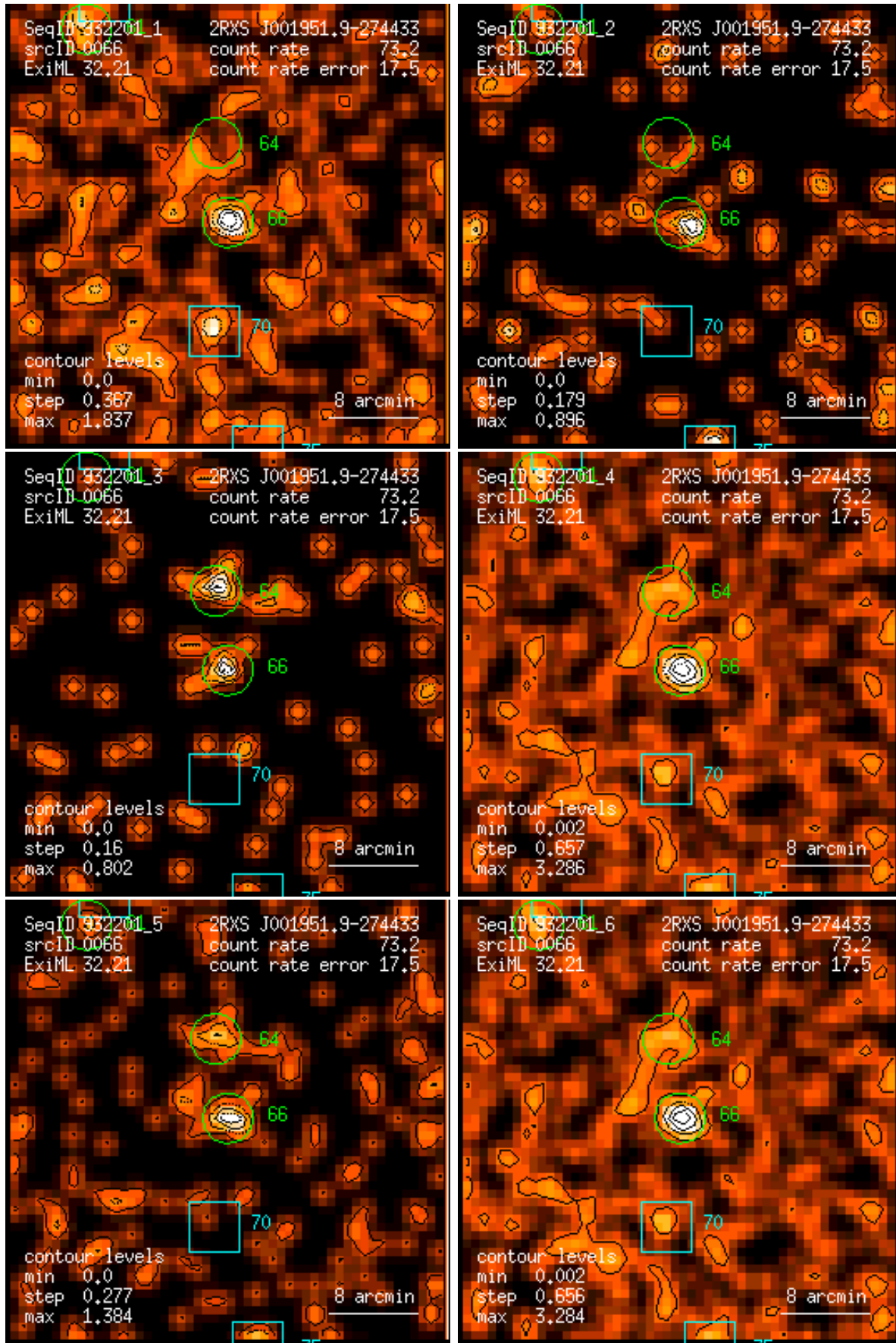
Figure 66: RASS 932201: detection 0066: band rate images, Gaussian filter: (1) PSPC channels 11 – 41, (2) 52 – 90, (3) 91 – 201, (4) 11 – 235, (5) 52 – 201, (6) 11 – 201. Broad band rates in counts/ks. Band rate contour levels in counts/ks/arcmin 2 .
