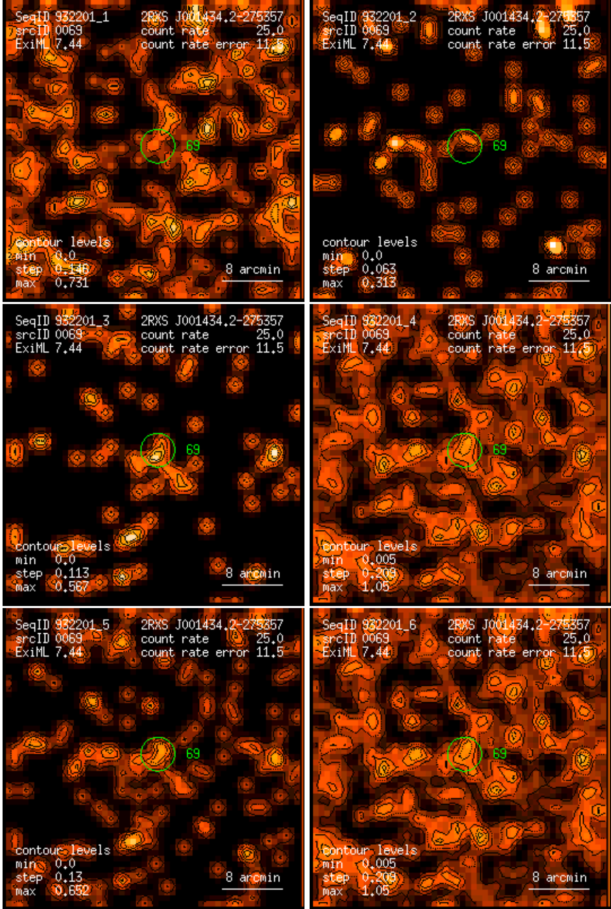
Figure 69: RASS 932201: detection 0069: band rate images, Gaussian filter: (1) PSPC channels 11 – 41, (2) 52 – 90, (3) 91 – 201, (4) 11 – 235, (5) 52 – 201, (6) 11 – 201. Broad band rates in counts/ks. Band rate contour levels in counts/ks/arcmin 2 .
