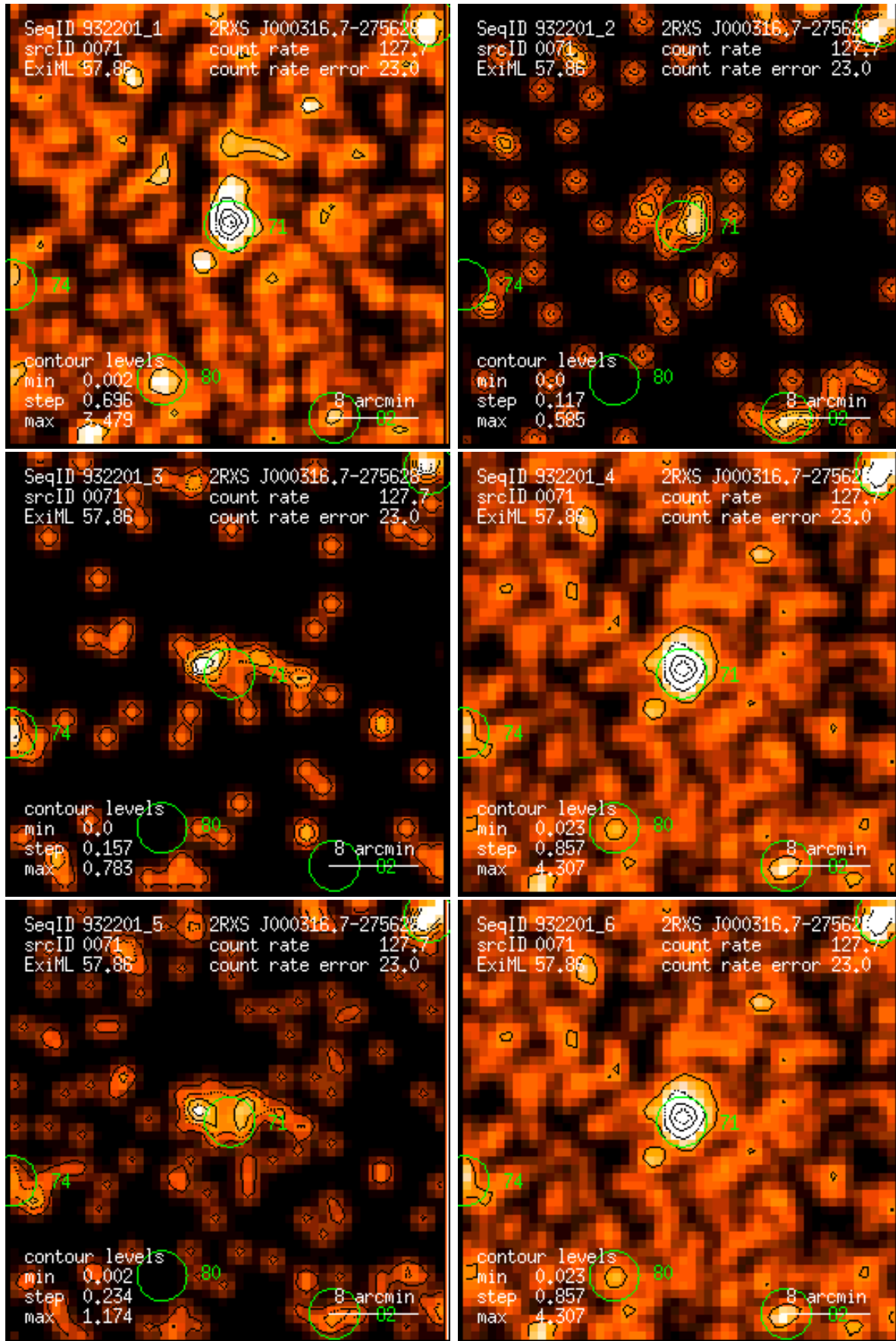
Figure 71: RASS 932201: detection 0071: band rate images, Gaussian filter: (1) PSPC channels 11 – 41, (2) 52 – 90, (3) 91 – 201, (4) 11 – 235, (5) 52 – 201, (6) 11 – 201. Broad band rates in counts/ks. Band rate contour levels in counts/ks/arcmin 2 .
