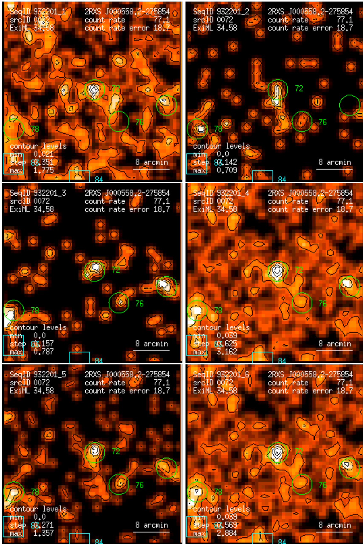
Figure 72: RASS 932201: detection 0072: band rate images, Gaussian filter: (1) PSPC channels 11 – 41, (2) 52 – 90, (3) 91 – 201, (4) 11 – 235, (5) 52 – 201, (6) 11 – 201. Broad band rates in counts/ks. Band rate contour levels in counts/ks/arcmin 2 .
