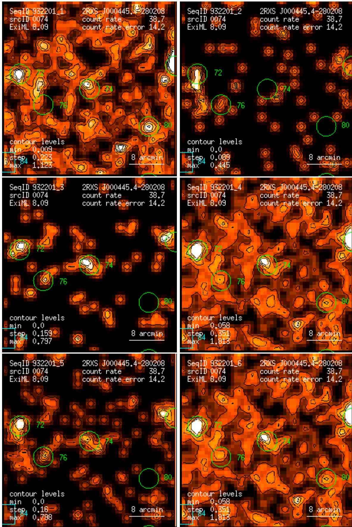
Figure 74: RASS 932201: detection 0074: band rate images, Gaussian filter: (1) PSPC channels 11 – 41, (2) 52 – 90, (3) 91 – 201, (4) 11 – 235, (5) 52 – 201, (6) 11 – 201. Broad band rates in counts/ks. Band rate contour levels in counts/ks/arcmin 2 .
