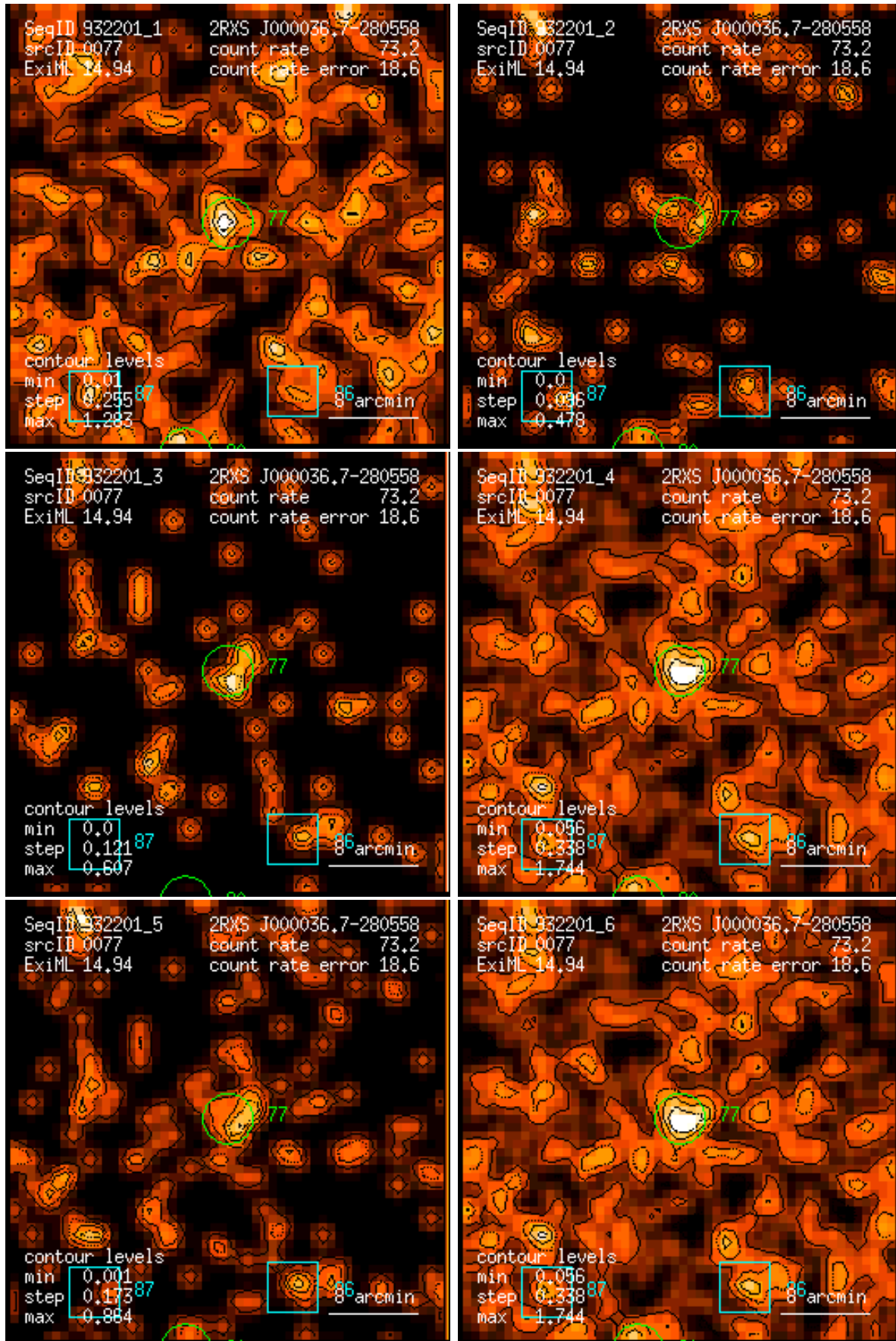
Figure 77: RASS 932201: detection 0077: band rate images, Gaussian filter: (1) PSPC channels 11 – 41, (2) 52 – 90, (3) 91 – 201, (4) 11 – 235, (5) 52 – 201, (6) 11 – 201. Broad band rates in counts/ks. Band rate contour levels in counts/ks/arcmin 2 .
