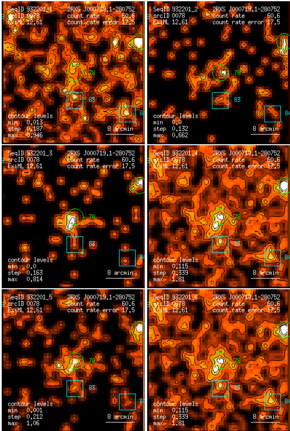
Figure 78: RASS 932201: detection 0078: band rate images, Gaussian filter: (1) PSPC channels 11 – 41, (2) 52 – 90, (3) 91 – 201, (4) 11 – 235, (5) 52 – 201, (6) 11 – 201. Broad band rates in counts/ks. Band rate contour levels in counts/ks/arcmin 2 .
