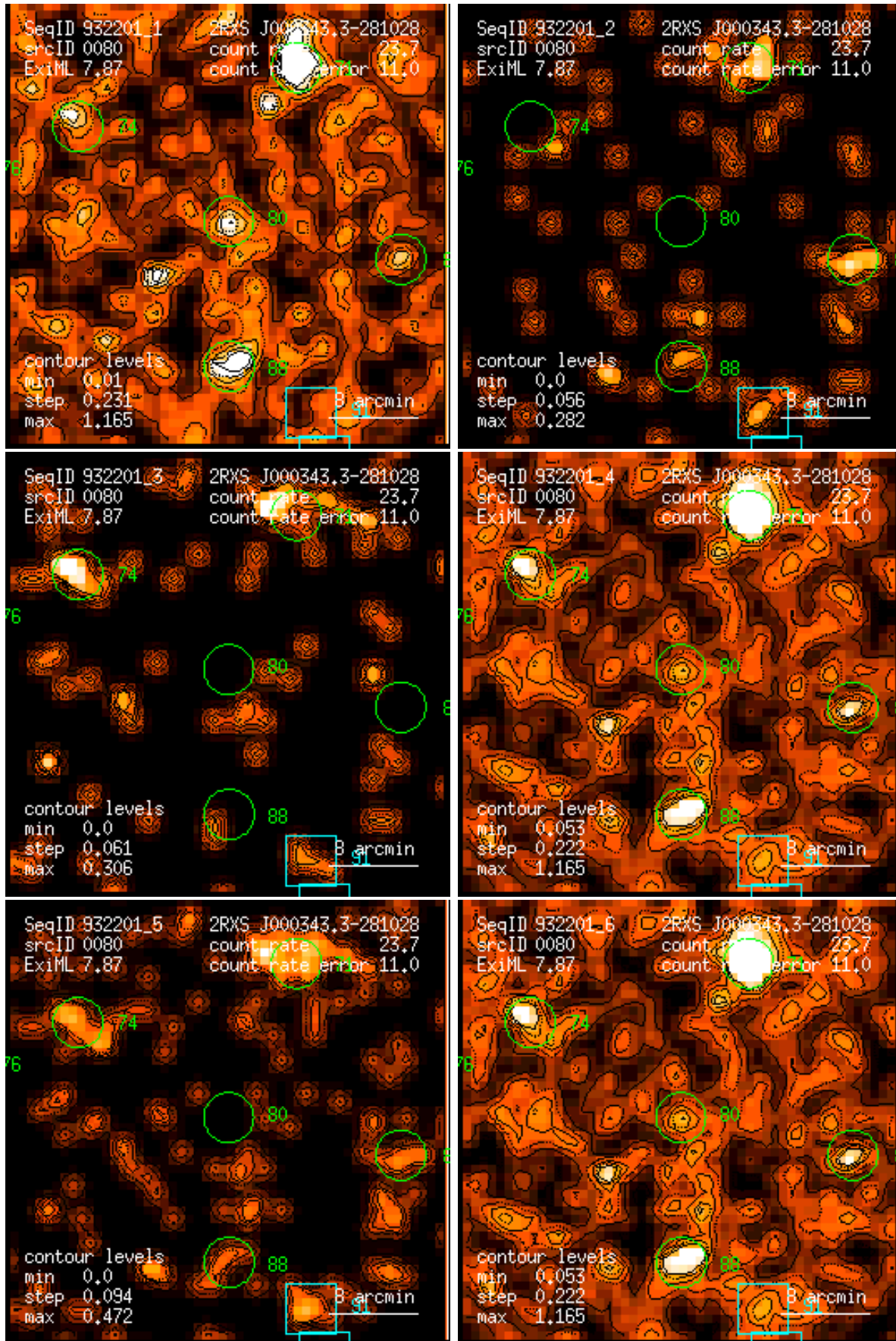
Figure 80: RASS 932201: detection 0080: band rate images, Gaussian filter: (1) PSPC channels 11 – 41, (2) 52 – 90, (3) 91 – 201, (4) 11 – 235, (5) 52 – 201, (6) 11 – 201. Broad band rates in counts/ks. Band rate contour levels in counts/ks/arcmin 2 .
