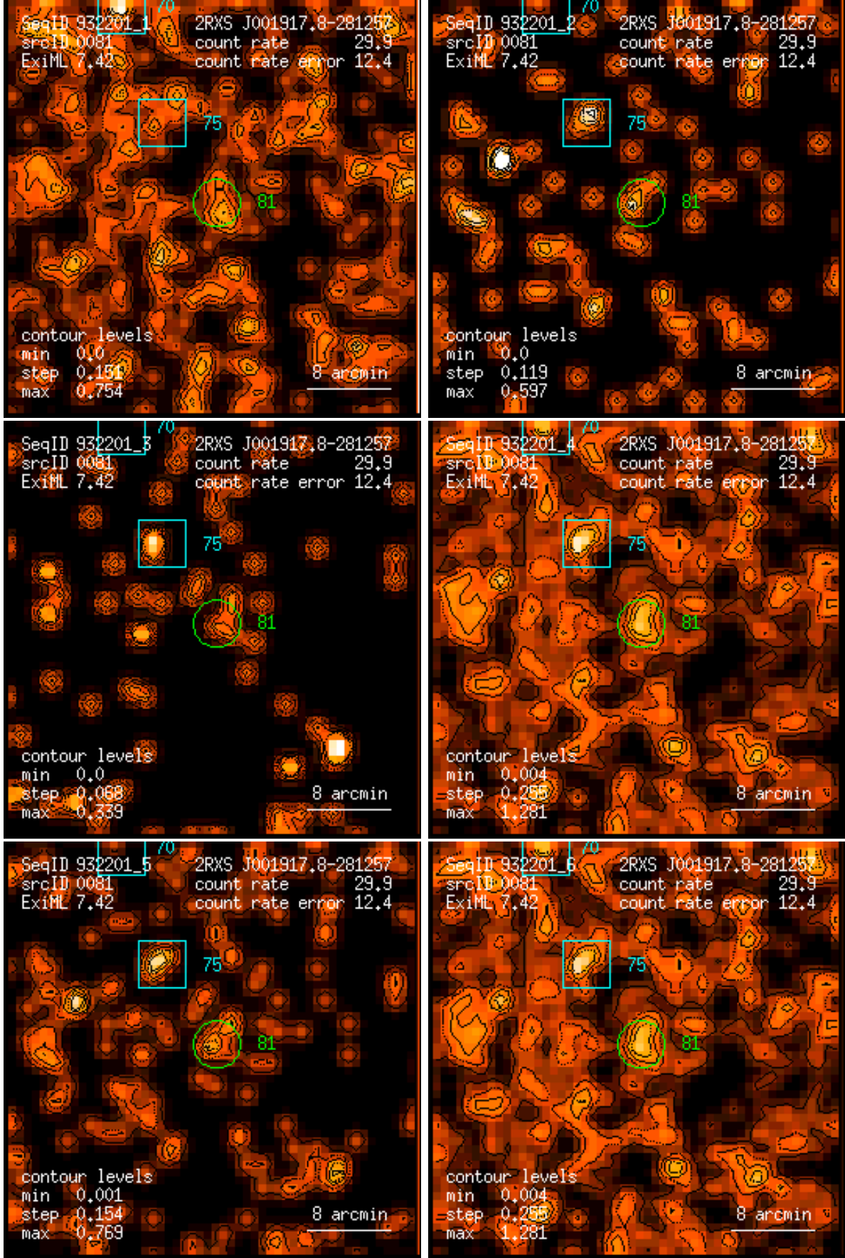
Figure 81: RASS 932201: detection 0081: band rate images, Gaussian filter: (1) PSPC channels 11 – 41, (2) 52 – 90, (3) 91 – 201, (4) 11 – 235, (5) 52 – 201, (6) 11 – 201. Broad band rates in counts/ks. Band rate contour levels in counts/ks/arcmin 2 .
