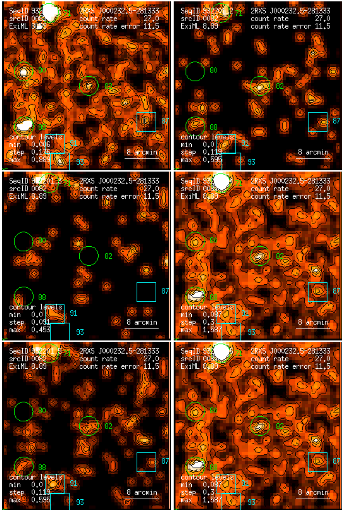
Figure 82: RASS 932201: detection 0082: band rate images, Gaussian filter: (1) PSPC channels 11 – 41, (2) 52 – 90, (3) 91 – 201, (4) 11 – 235, (5) 52 – 201, (6) 11 – 201. Broad band rates in counts/ks. Band rate contour levels in counts/ks/arcmin 2 .
