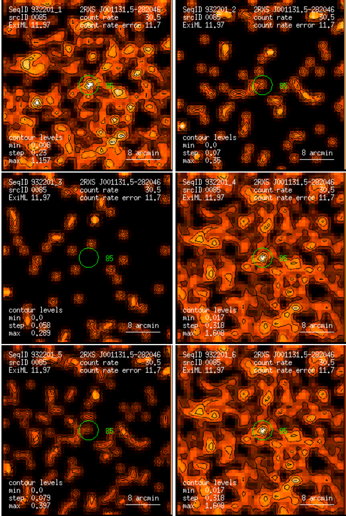
Figure 85: RASS 932201: detection 0085: band rate images, Gaussian filter: (1) PSPC channels 11 – 41, (2) 52 – 90, (3) 91 – 201, (4) 11 – 235, (5) 52 – 201, (6) 11 – 201. Broad band rates in counts/ks. Band rate contour levels in counts/ks/arcmin 2 .
