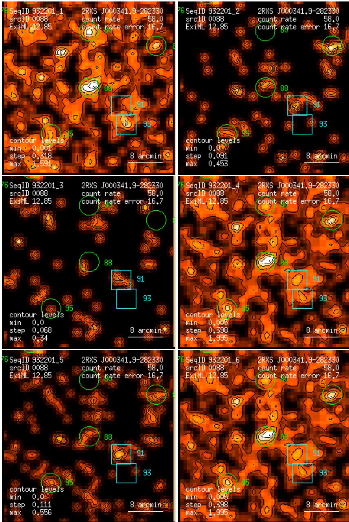
Figure 88: RASS 932201: detection 0088: band rate images, Gaussian filter: (1) PSPC channels 11 – 41, (2) 52 – 90, (3) 91 – 201, (4) 11 – 235, (5) 52 – 201, (6) 11 – 201. Broad band rates in counts/ks. Band rate contour levels in counts/ks/arcmin 2 .
