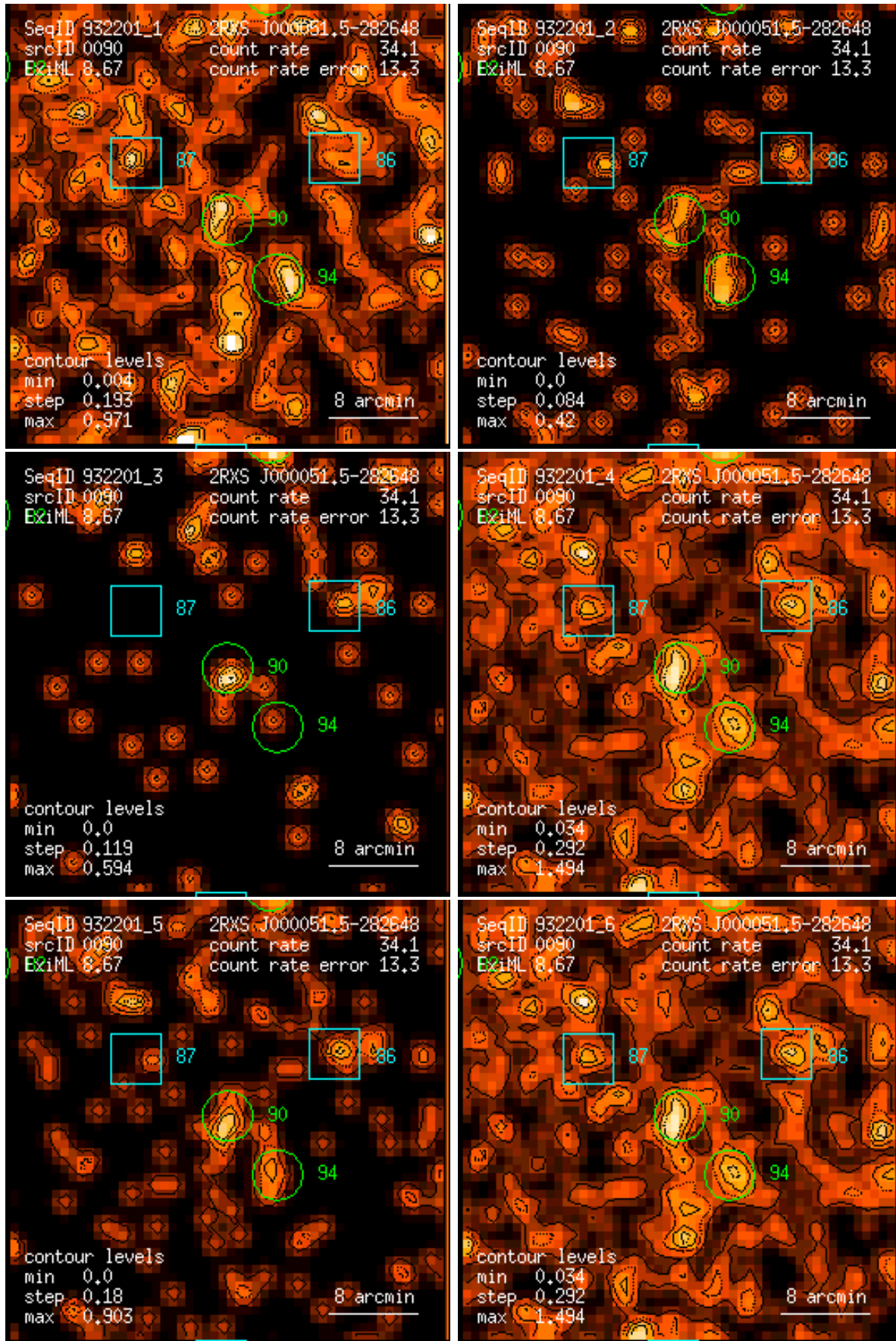
Figure 90: RASS 932201: detection 0090: band rate images, Gaussian filter: (1) PSPC channels 11 – 41, (2) 52 – 90, (3) 91 – 201, (4) 11 – 235, (5) 52 – 201, (6) 11 – 201. Broad band rates in counts/ks. Band rate contour levels in counts/ks/arcmin 2 .
