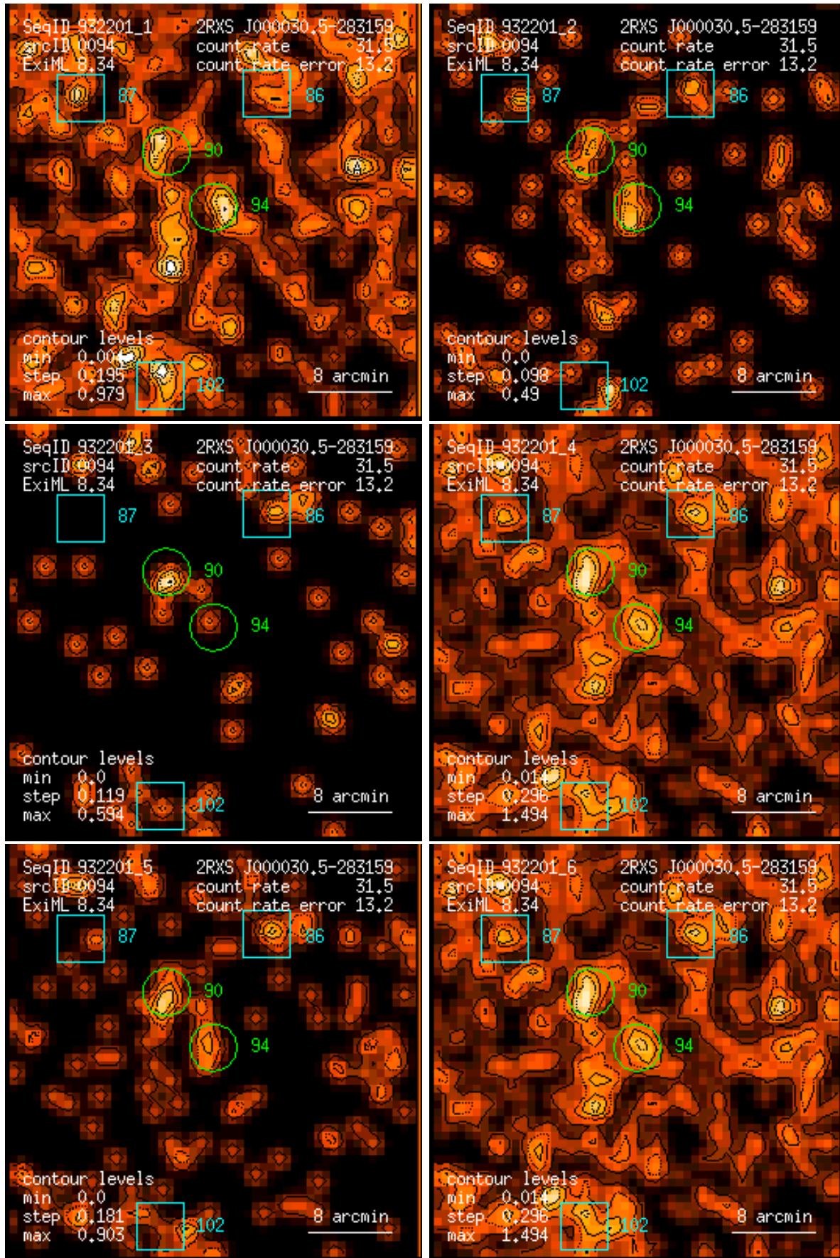
Figure 94: RASS 932201: detection 0094: band rate images, Gaussian filter: (1) PSPC channels 11 – 41, (2) 52 – 90, (3) 91 – 201, (4) 11 – 235, (5) 52 – 201, (6) 11 – 201. Broad band rates in counts/ks. Band rate contour levels in counts/ks/arcmin 2 .
