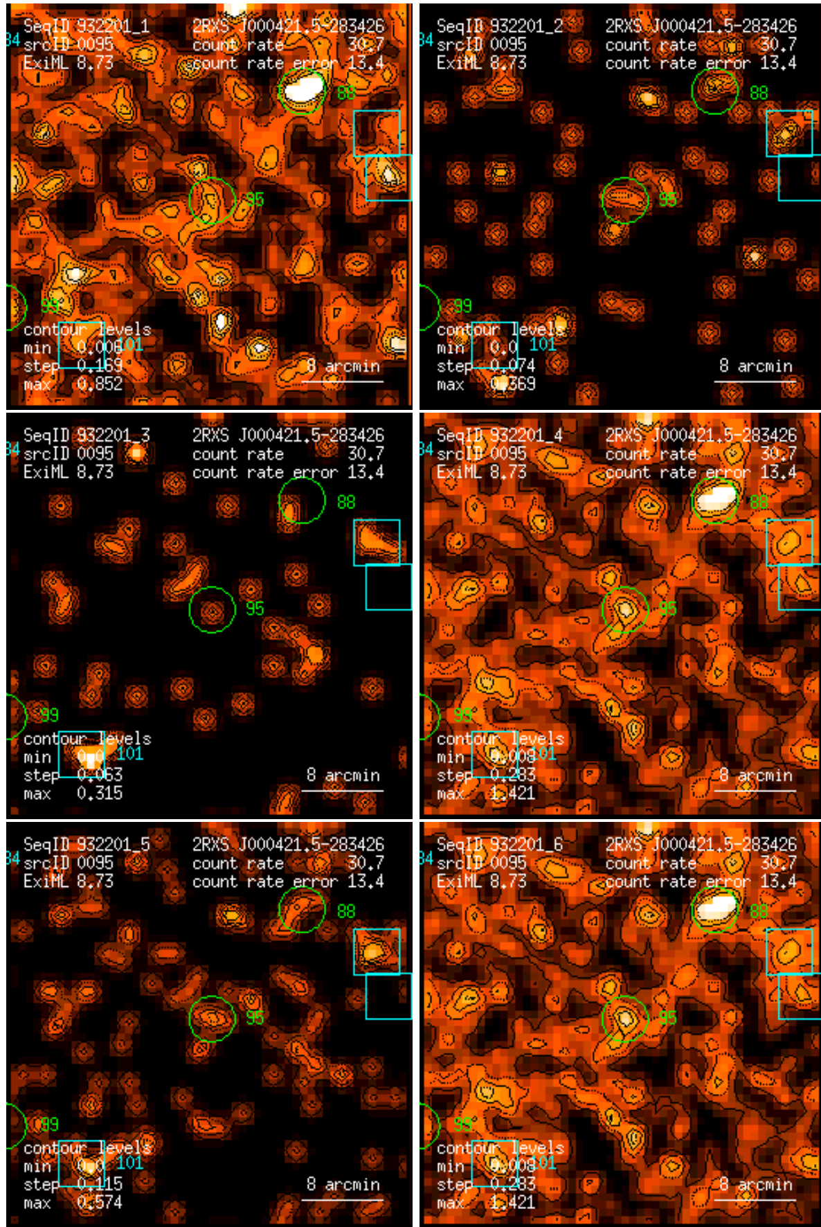
Figure 95: RASS 932201: detection 0095: band rate images, Gaussian filter: (1) PSPC channels 11 – 41, (2) 52 – 90, (3) 91 – 201, (4) 11 – 235, (5) 52 – 201, (6) 11 – 201. Broad band rates in counts/ks. Band rate contour levels in counts/ks/arcmin 2 .
