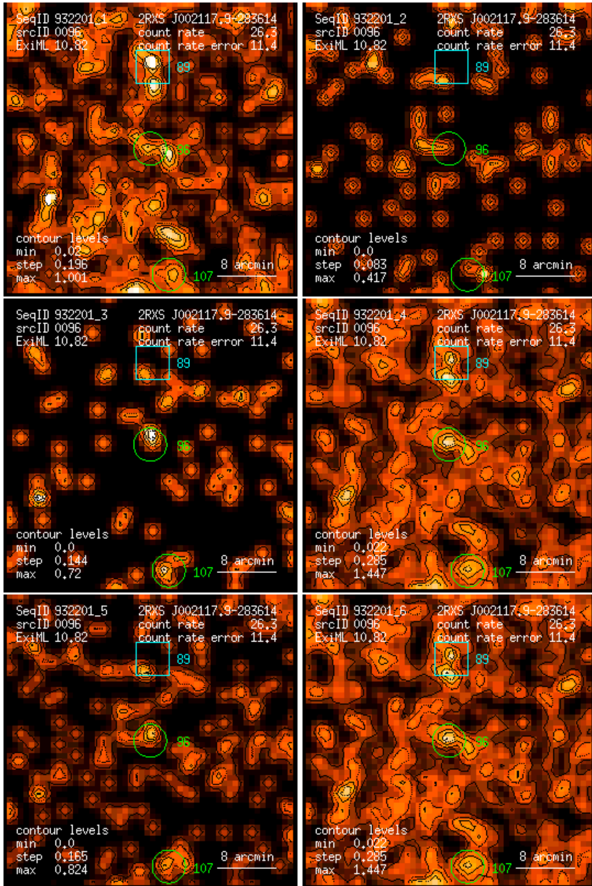
Figure 96: RASS 932201: detection 0096: band rate images, Gaussian filter: (1) PSPC channels 11 – 41, (2) 52 – 90, (3) 91 – 201, (4) 11 – 235, (5) 52 – 201, (6) 11 – 201. Broad band rates in counts/ks. Band rate contour levels in counts/ks/arcmin 2 .
