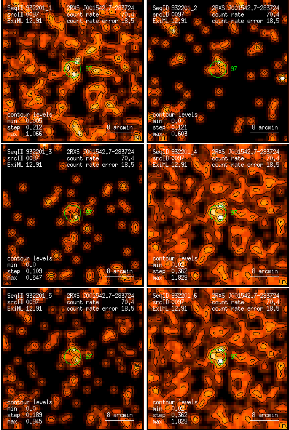
Figure 97: RASS 932201: detection 0097: band rate images, Gaussian filter: (1) PSPC channels 11 – 41, (2) 52 – 90, (3) 91 – 201, (4) 11 – 235, (5) 52 – 201, (6) 11 – 201. Broad band rates in counts/ks. Band rate contour levels in counts/ks/arcmin 2 .
