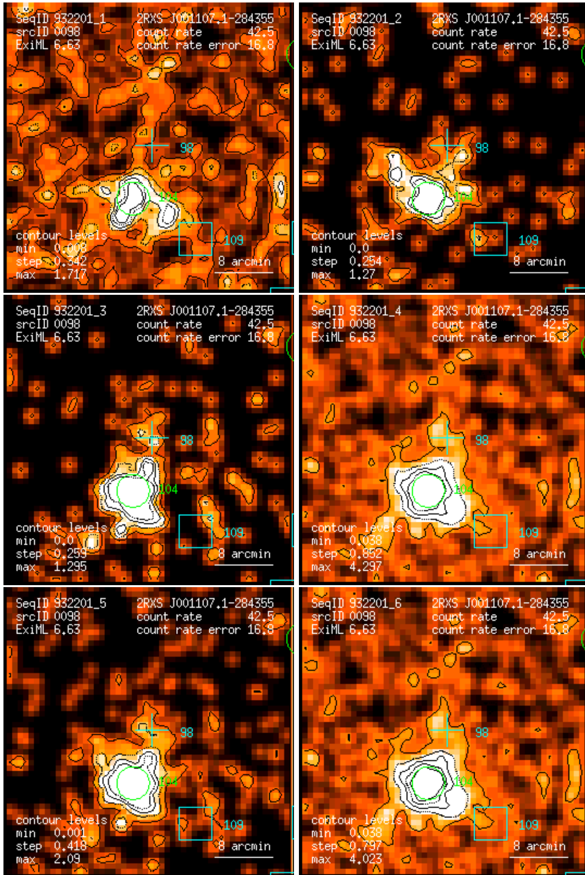
Figure 98: RASS 932201: detection 0098: band rate images, Gaussian filter: (1) PSPC channels 11 – 41, (2) 52 – 90, (3) 91 – 201, (4) 11 – 235, (5) 52 – 201, (6) 11 – 201. Broad band rates in counts/ks. Band rate contour levels in counts/ks/arcmin 2 .
