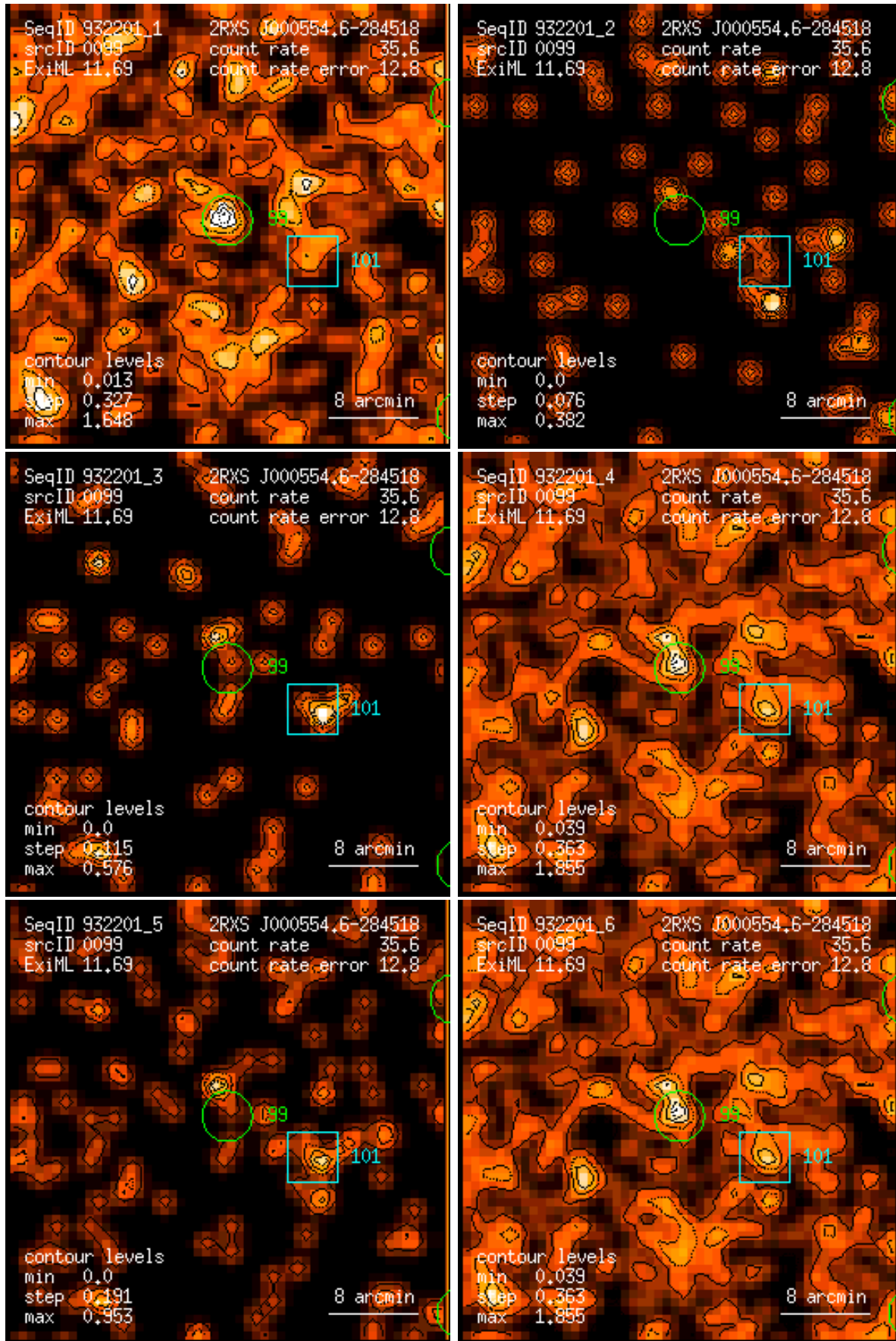
Figure 99: RASS 932201: detection 0099: band rate images, Gaussian filter: (1) PSPC channels 11 – 41, (2) 52 – 90, (3) 91 – 201, (4) 11 – 235, (5) 52 – 201, (6) 11 – 201. Broad band rates in counts/ks. Band rate contour levels in counts/ks/arcmin 2 .
