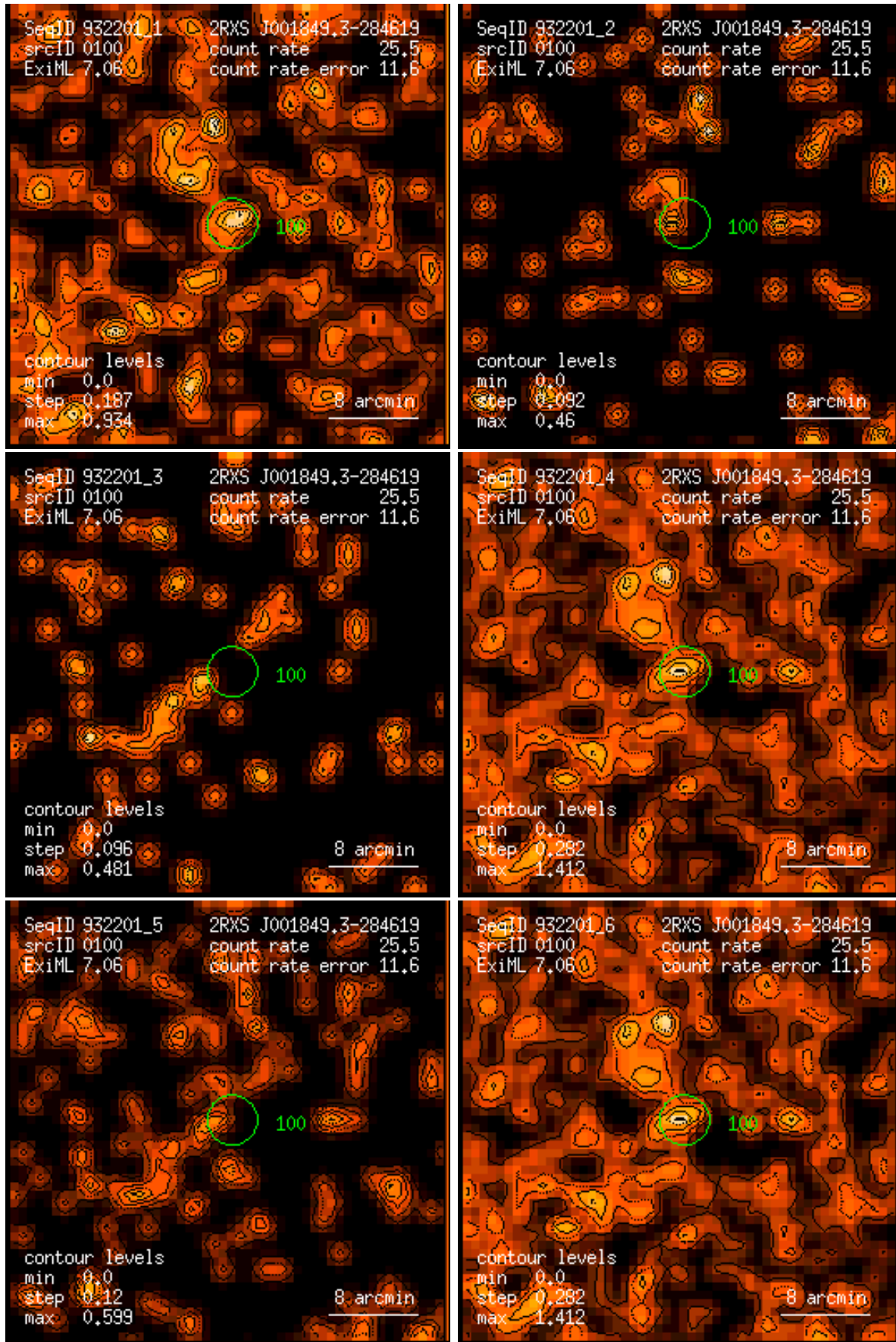
Figure 100: RASS 932201: detection 0100: band rate images, Gaussian filter: (1) PSPC channels 11 – 41, (2) 52 – 90, (3) 91 – 201, (4) 11 – 235, (5) 52 – 201, (6) 11 – 201. Broad band rates in counts/ks. Band rate contour levels in counts/ks/arcmin 2 .
