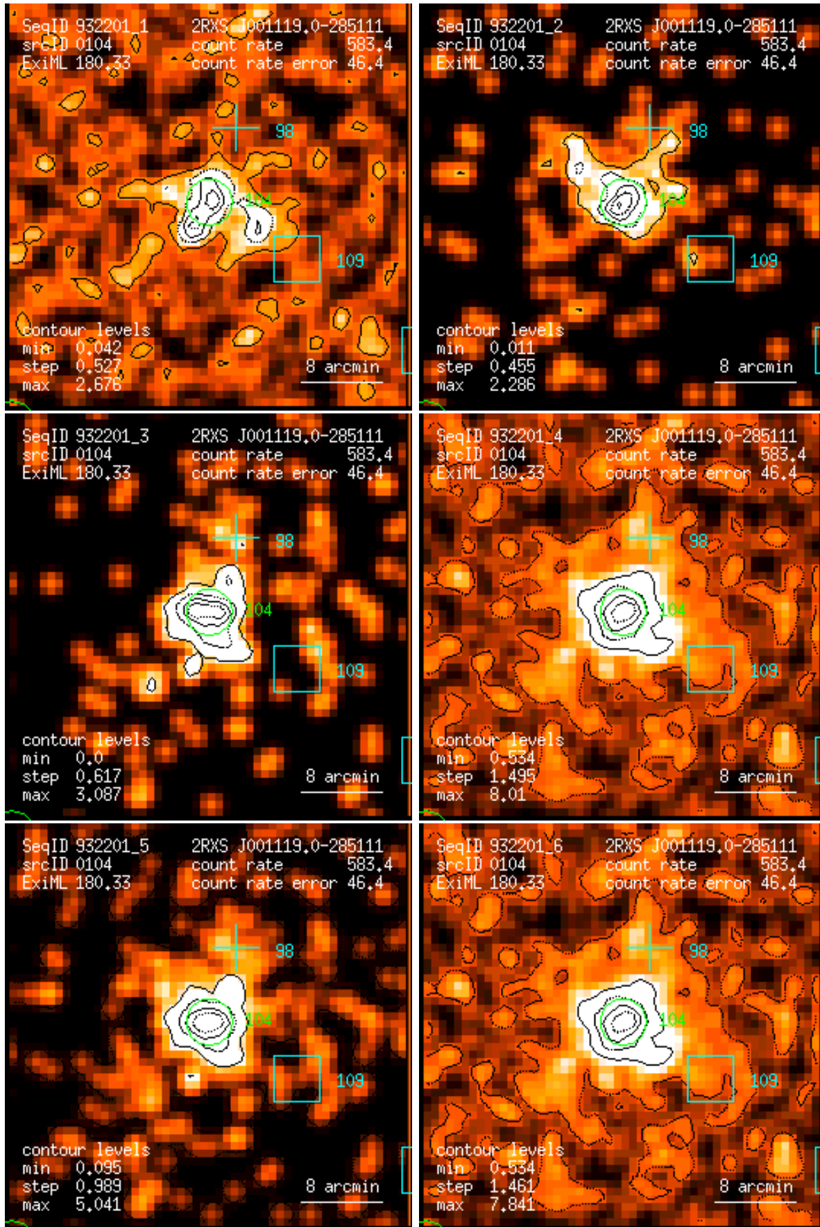
Figure 104: RASS 932201: detection 0104: band rate images, Gaussian filter: (1) PSPC channels 11 – 41, (2) 52 – 90, (3) 91 – 201, (4) 11 – 235, (5) 52 – 201, (6) 11 – 201. Broad band rates in counts/ks. Band rate contour levels in counts/ks/arcmin 2 .
