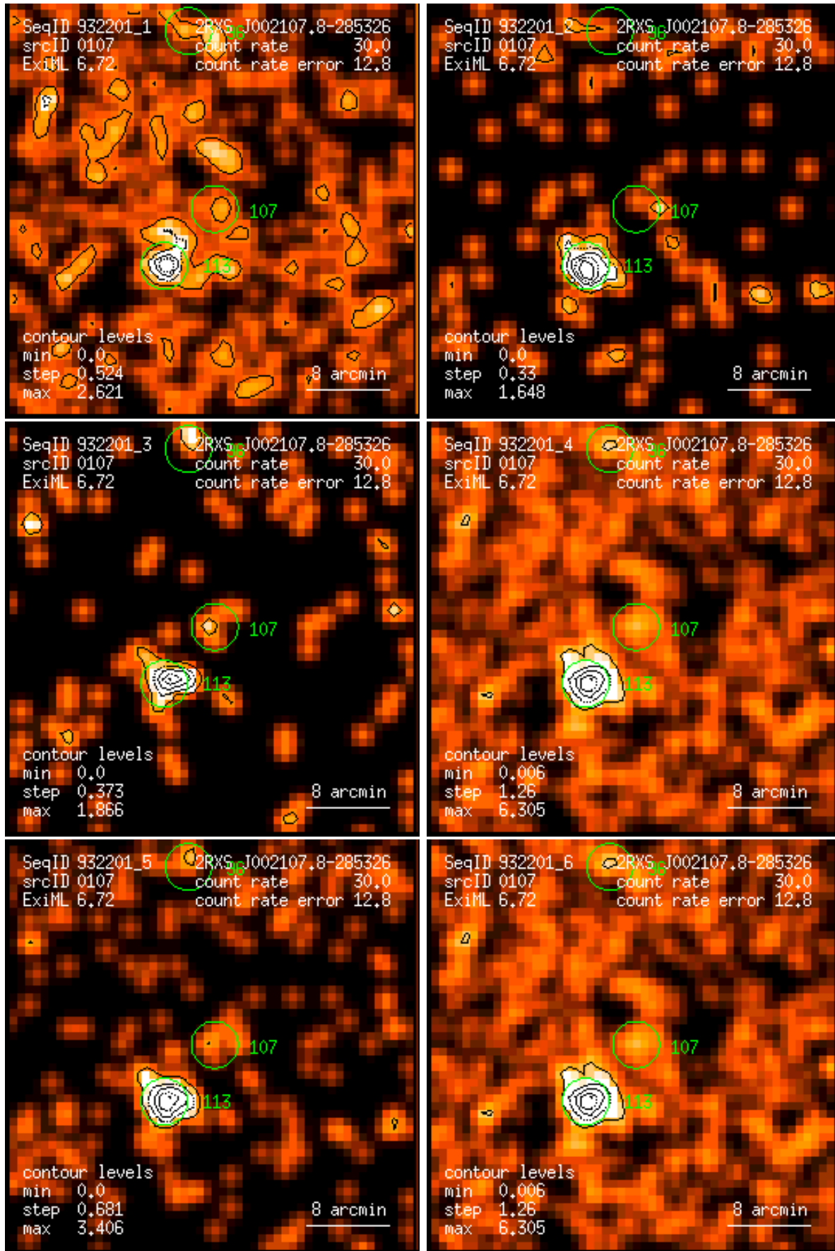
Figure 107: RASS 932201: detection 0107: band rate images, Gaussian filter: (1) PSPC channels 11 – 41, (2) 52 – 90, (3) 91 – 201, (4) 11 – 235, (5) 52 – 201, (6) 11 – 201. Broad band rates in counts/ks. Band rate contour levels in counts/ks/arcmin 2 .
