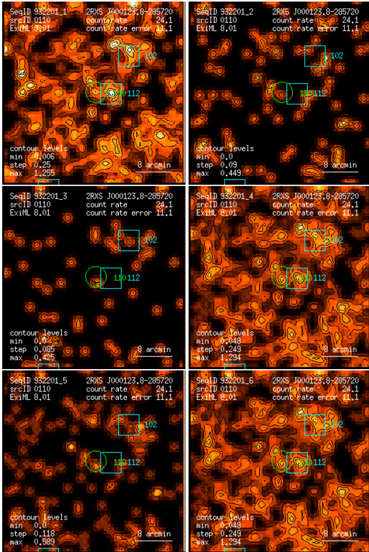
Figure 110: RASS 932201: detection 0110: band rate images, Gaussian filter: (1) PSPC channels 11 – 41, (2) 52 – 90, (3) 91 – 201, (4) 11 – 235, (5) 52 – 201, (6) 11 – 201. Broad band rates in counts/ks. Band rate contour levels in counts/ks/arcmin 2 .
