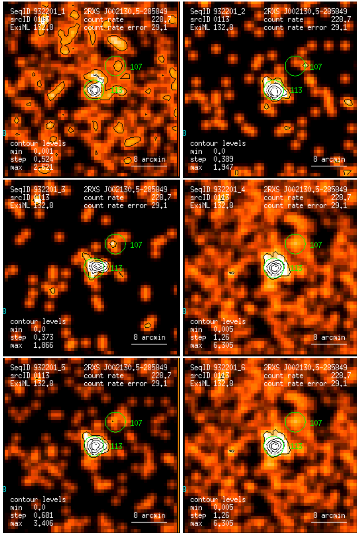
Figure 113: RASS 932201: detection 0113: band rate images, Gaussian filter: (1) PSPC channels 11 – 41, (2) 52 – 90, (3) 91 – 201, (4) 11 – 235, (5) 52 – 201, (6) 11 – 201. Broad band rates in counts/ks. Band rate contour levels in counts/ks/arcmin 2 .
