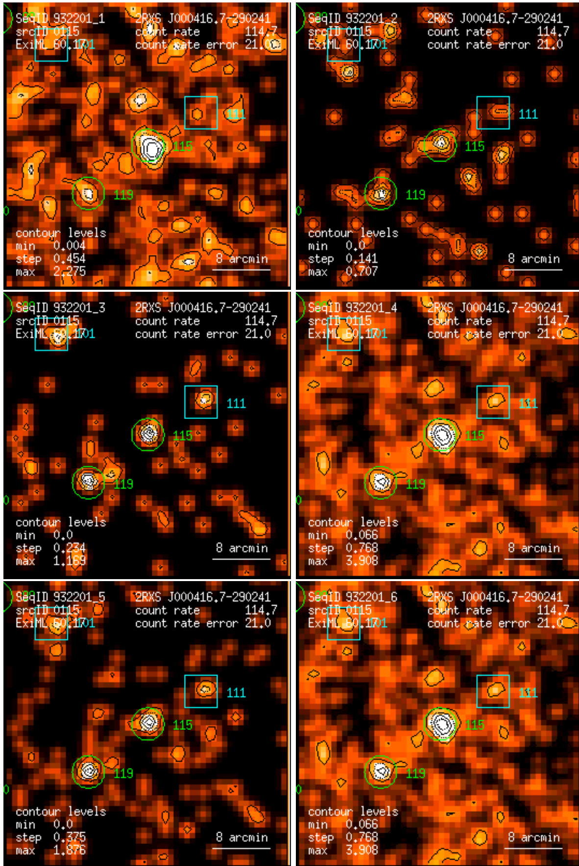
Figure 115: RASS 932201: detection 0115: band rate images, Gaussian filter: (1) PSPC channels 11 – 41, (2) 52 – 90, (3) 91 – 201, (4) 11 – 235, (5) 52 – 201, (6) 11 – 201. Broad band rates in counts/ks. Band rate contour levels in counts/ks/arcmin 2 .
