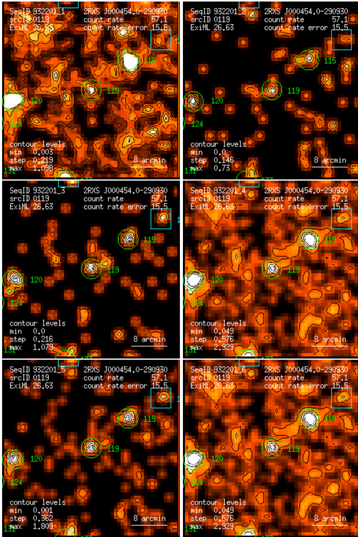
Figure 119: RASS 932201: detection 0119: band rate images, Gaussian filter: (1) PSPC channels 11 – 41, (2) 52 – 90, (3) 91 – 201, (4) 11 – 235, (5) 52 – 201, (6) 11 – 201. Broad band rates in counts/ks. Band rate contour levels in counts/ks/arcmin 2 .
