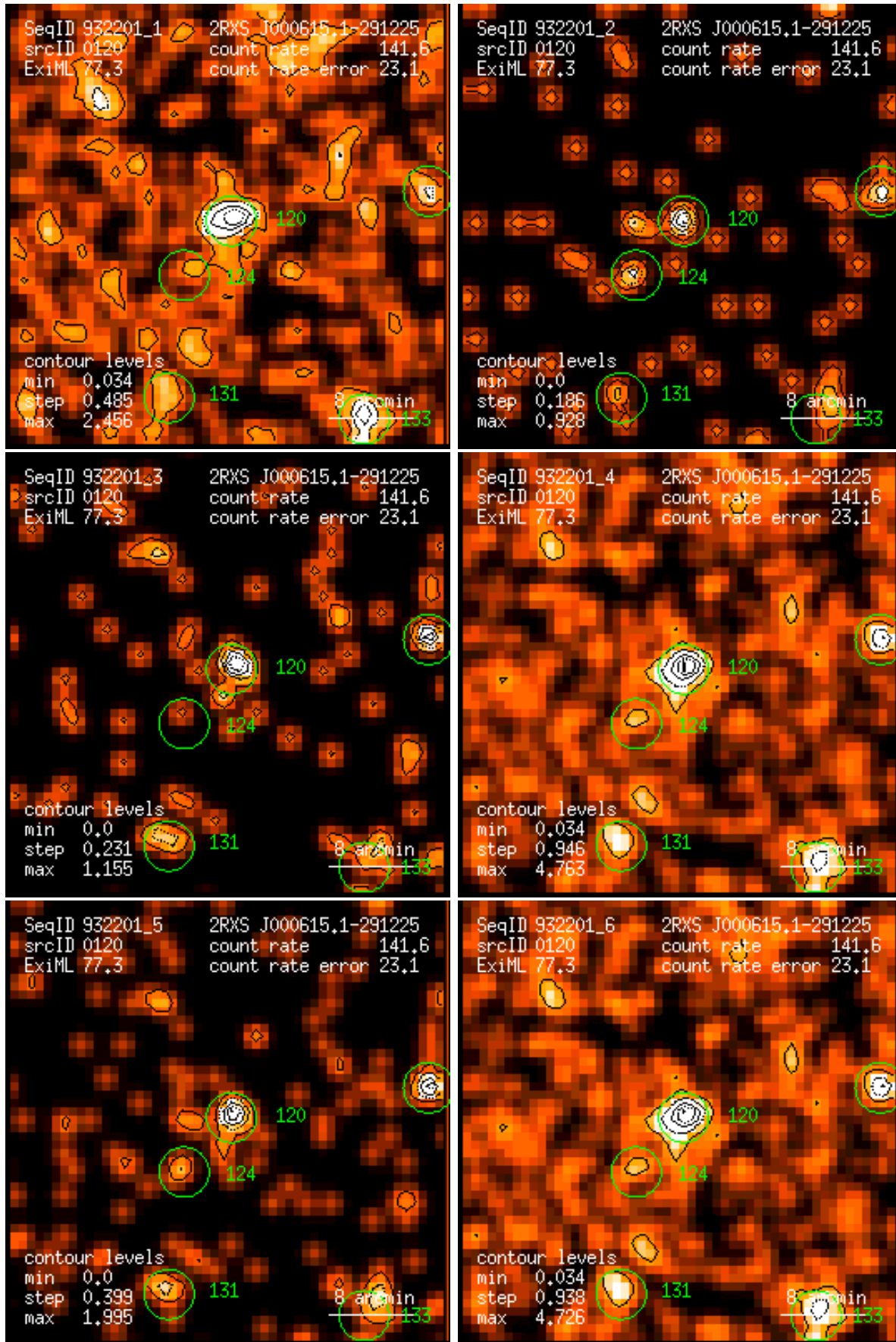
Figure 120: RASS 932201: detection 0120: band rate images, Gaussian filter: (1) PSPC channels 11 – 41, (2) 52 – 90, (3) 91 – 201, (4) 11 – 235, (5) 52 – 201, (6) 11 – 201. Broad band rates in counts/ks. Band rate contour levels in counts/ks/arcmin 2 .
