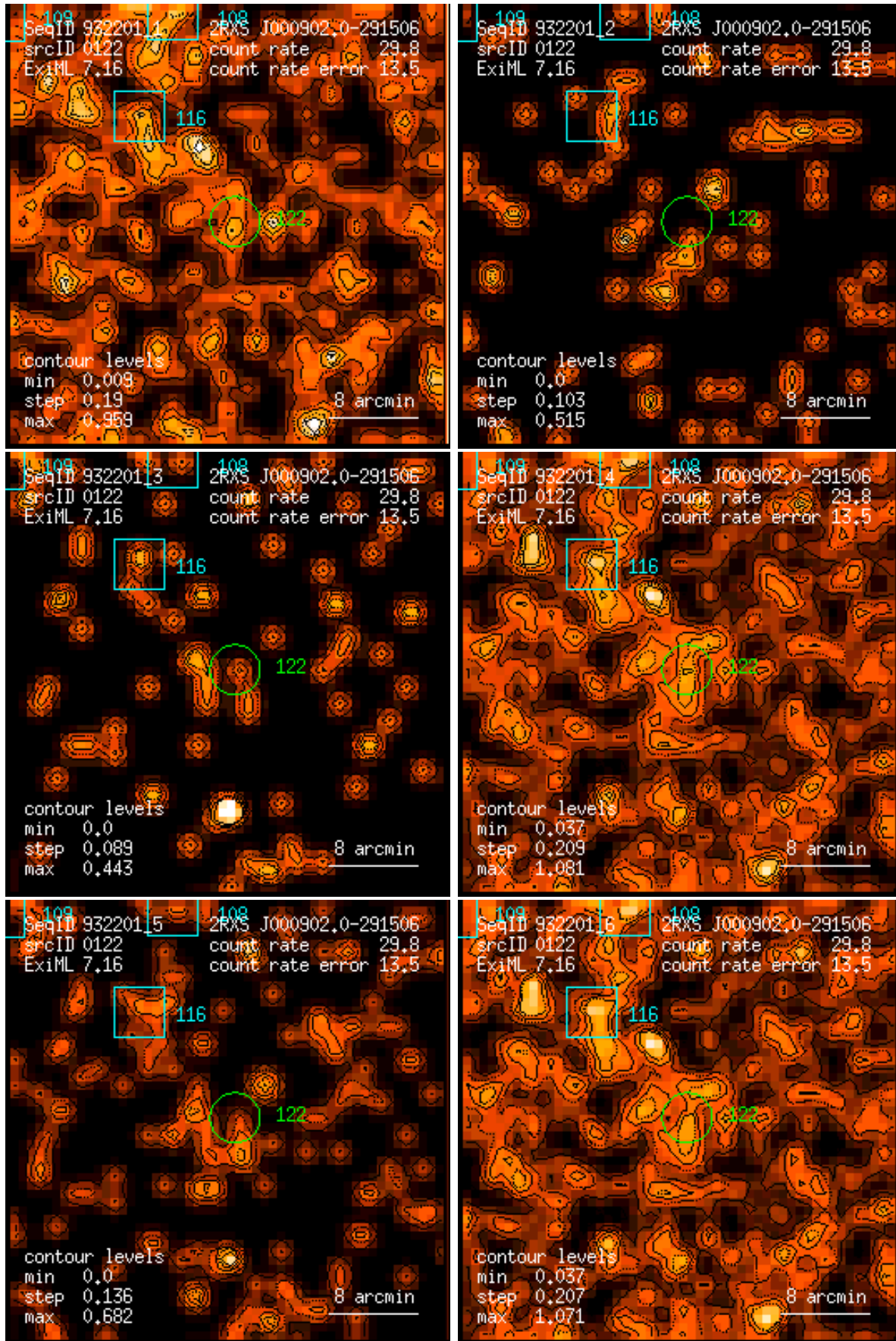
Figure 122: RASS 932201: detection 0122: band rate images, Gaussian filter: (1) PSPC channels 11 – 41, (2) 52 – 90, (3) 91 – 201, (4) 11 – 235, (5) 52 – 201, (6) 11 – 201. Broad band rates in counts/ks. Band rate contour levels in counts/ks/arcmin 2 .
