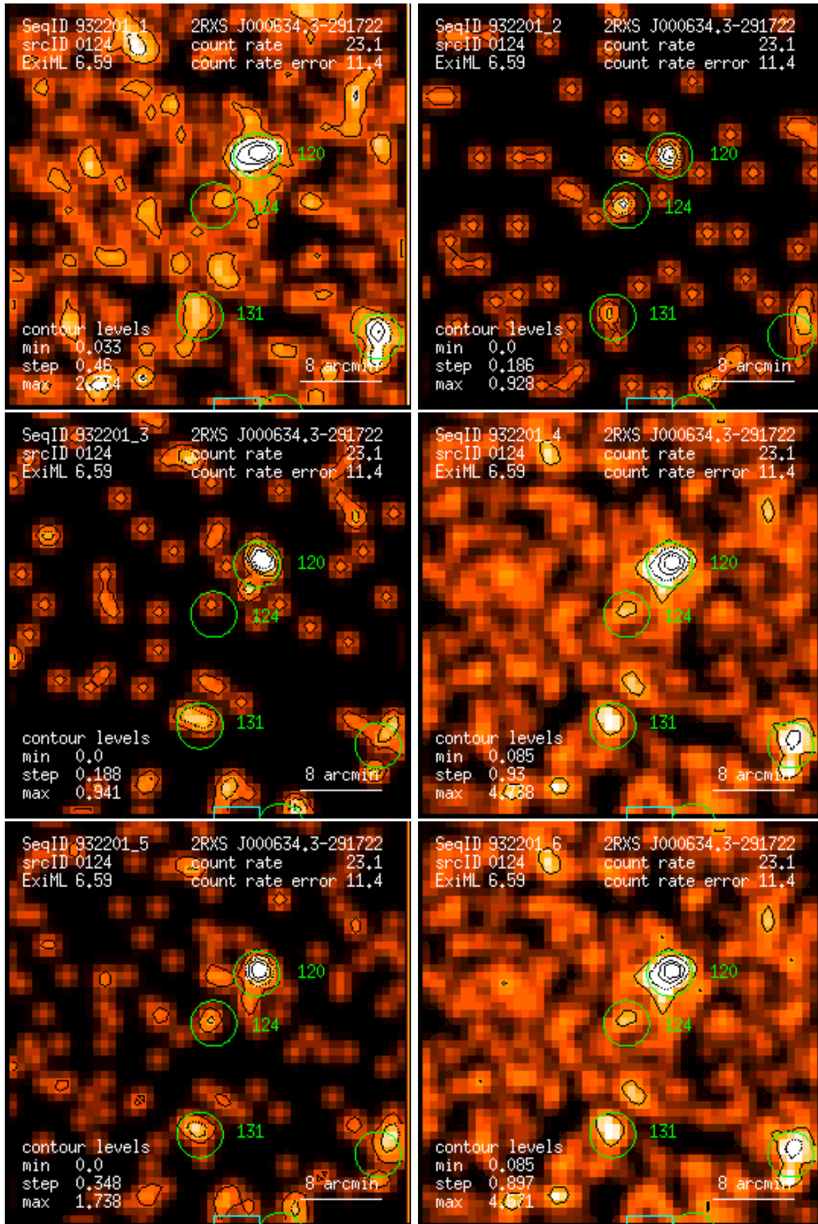
Figure 124: RASS 932201: detection 0124: band rate images, Gaussian filter: (1) PSPC channels 11 – 41, (2) 52 – 90, (3) 91 – 201, (4) 11 – 235, (5) 52 – 201, (6) 11 – 201. Broad band rates in counts/ks. Band rate contour levels in counts/ks/arcmin 2 .
