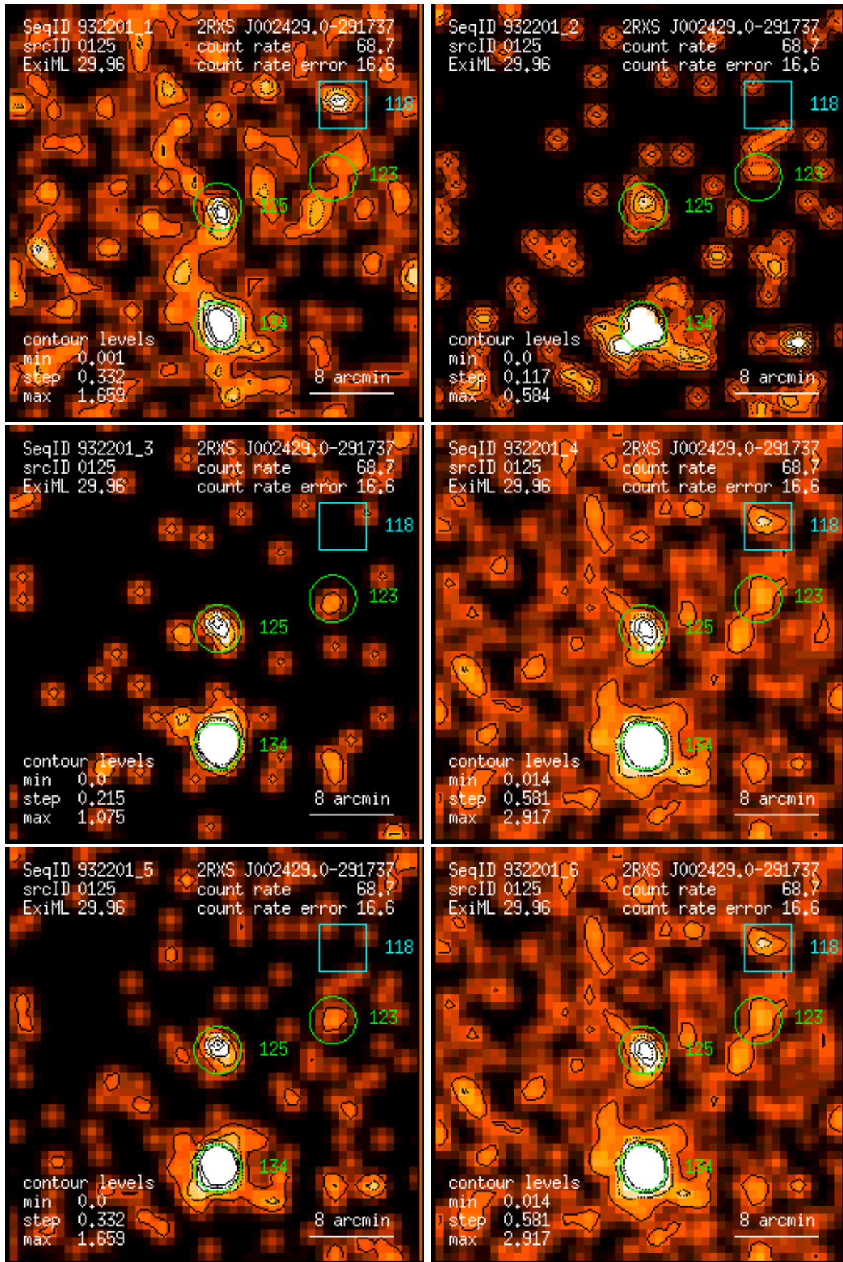
Figure 125: RASS 932201: detection 0125: band rate images, Gaussian filter: (1) PSPC channels 11 – 41, (2) 52 – 90, (3) 91 – 201, (4) 11 – 235, (5) 52 – 201, (6) 11 – 201. Broad band rates in counts/ks. Band rate contour levels in counts/ks/arcmin 2 .
