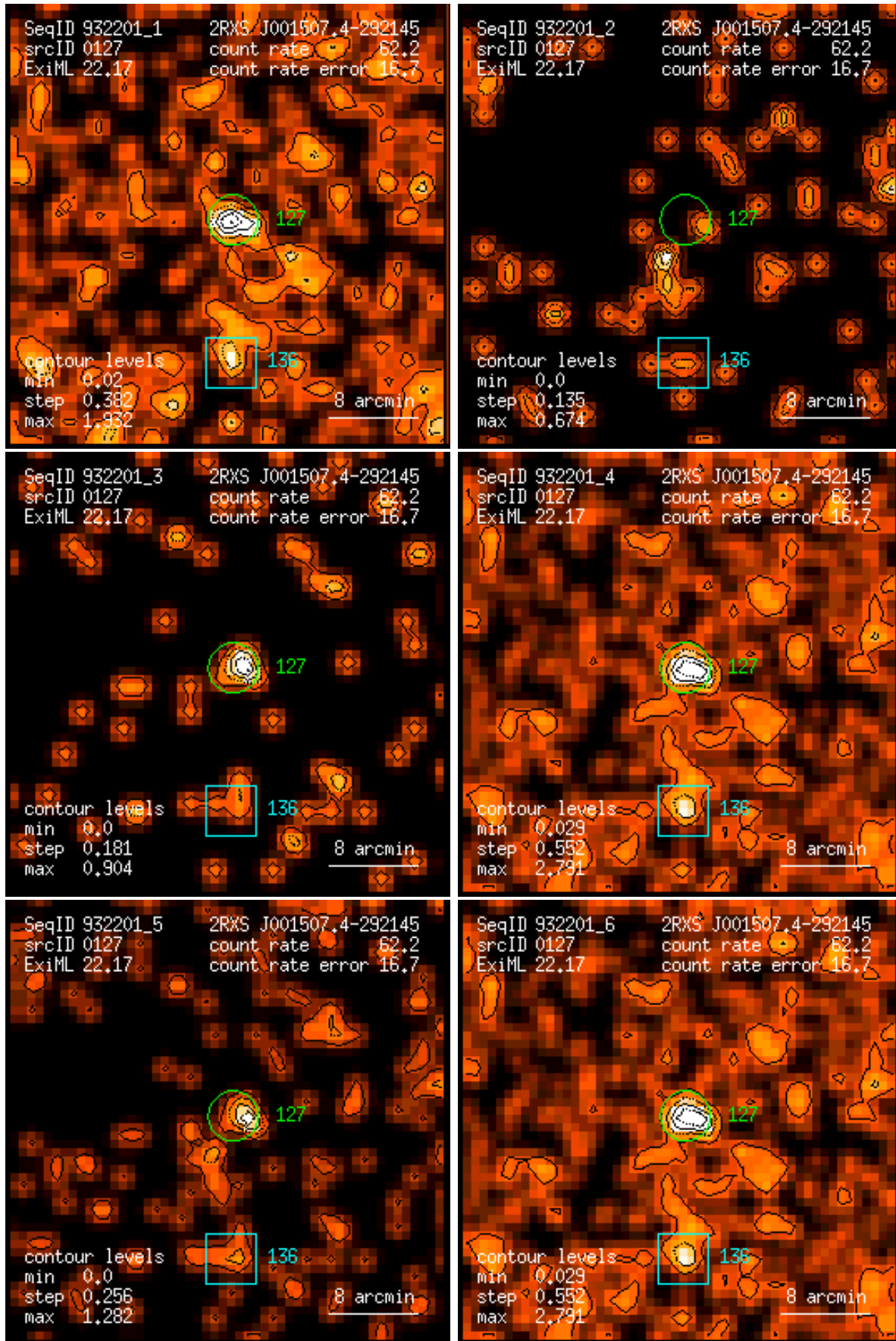
Figure 127: RASS 932201: detection 0127: band rate images, Gaussian filter: (1) PSPC channels 11 – 41, (2) 52 – 90, (3) 91 – 201, (4) 11 – 235, (5) 52 – 201, (6) 11 – 201. Broad band rates in counts/ks. Band rate contour levels in counts/ks/arcmin 2 .
