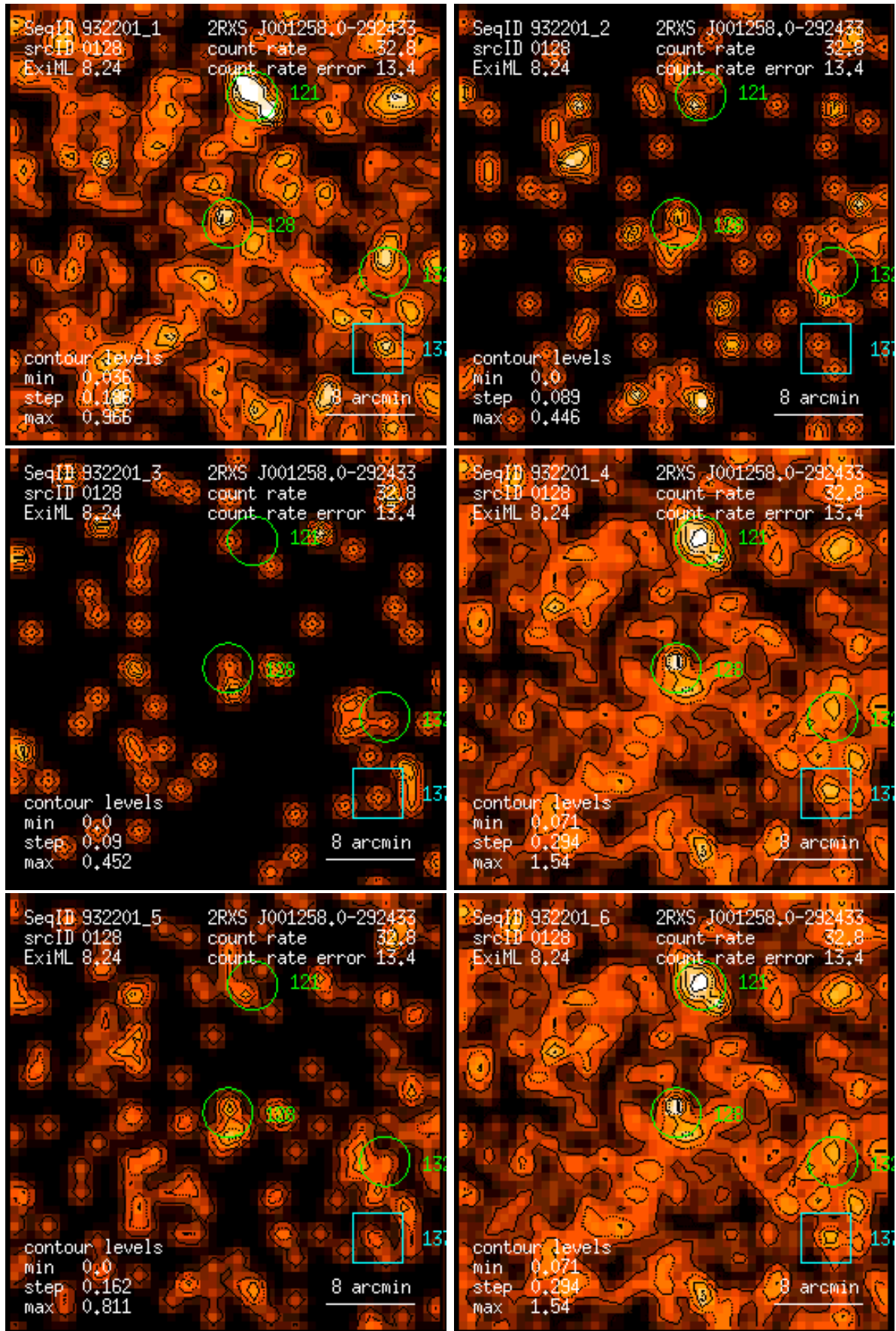
Figure 128: RASS 932201: detection 0128: band rate images, Gaussian filter: (1) PSPC channels 11 – 41, (2) 52 – 90, (3) 91 – 201, (4) 11 – 235, (5) 52 – 201, (6) 11 – 201. Broad band rates in counts/ks. Band rate contour levels in counts/ks/arcmin 2 .
