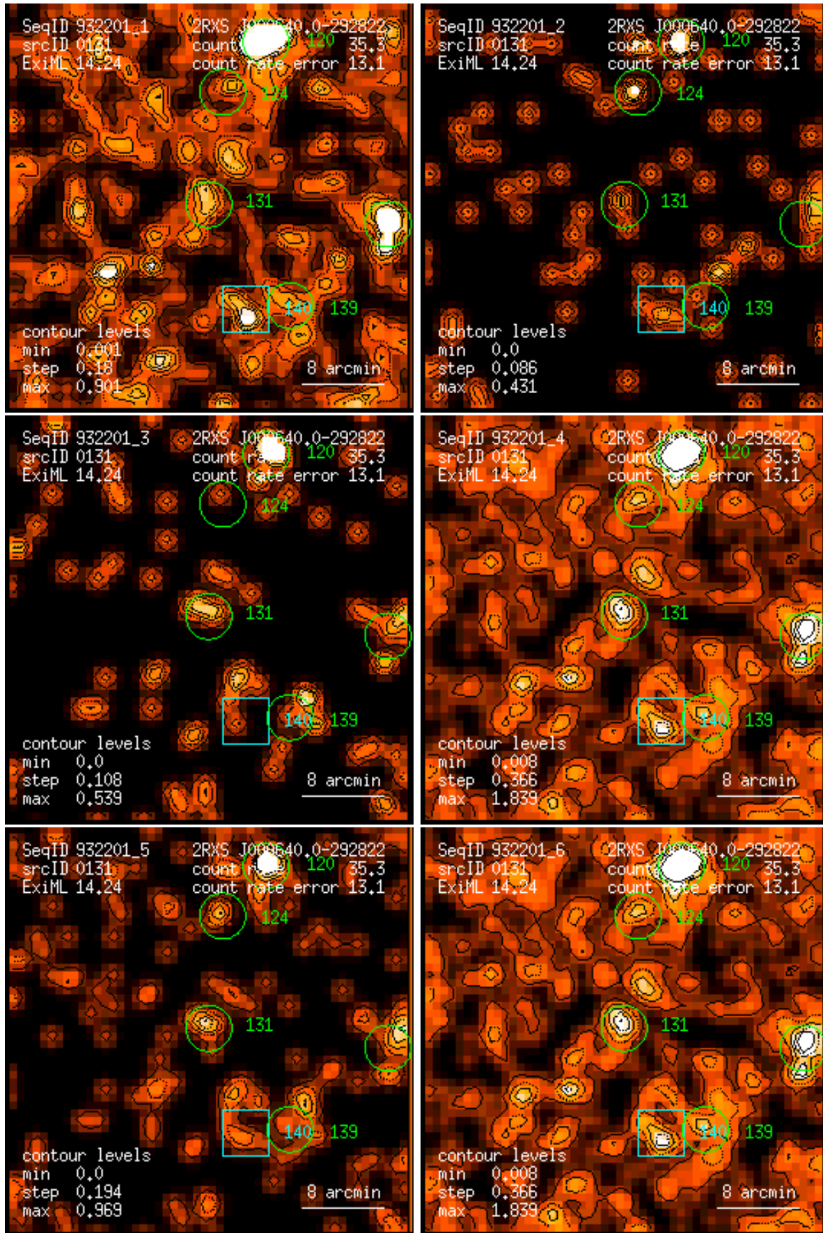
Figure 131: RASS 932201: detection 0131: band rate images, Gaussian filter: (1) PSPC channels 11 – 41, (2) 52 – 90, (3) 91 – 201, (4) 11 – 235, (5) 52 – 201, (6) 11 – 201. Broad band rates in counts/ks. Band rate contour levels in counts/ks/arcmin 2 .
