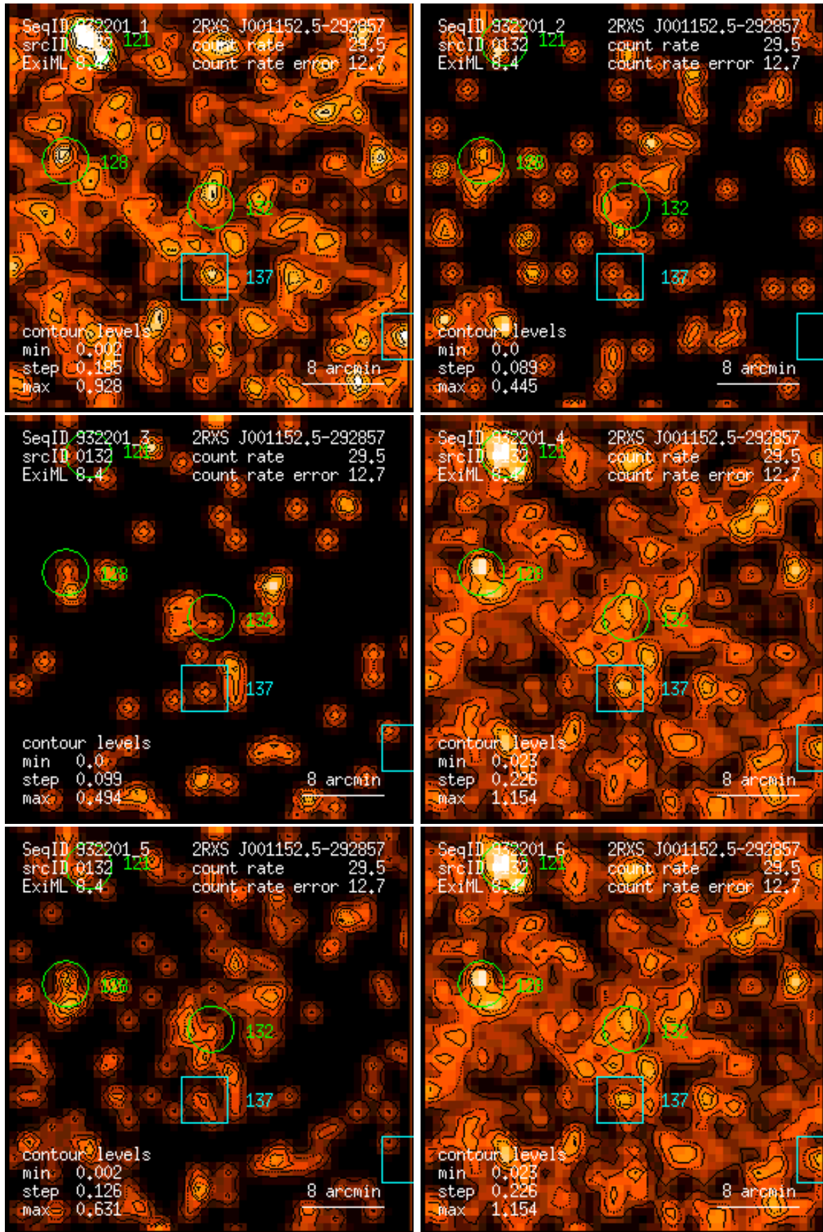
Figure 132: RASS 932201: detection 0132: band rate images, Gaussian filter: (1) PSPC channels 11 – 41, (2) 52 – 90, (3) 91 – 201, (4) 11 – 235, (5) 52 – 201, (6) 11 – 201. Broad band rates in counts/ks. Band rate contour levels in counts/ks/arcmin 2 .
