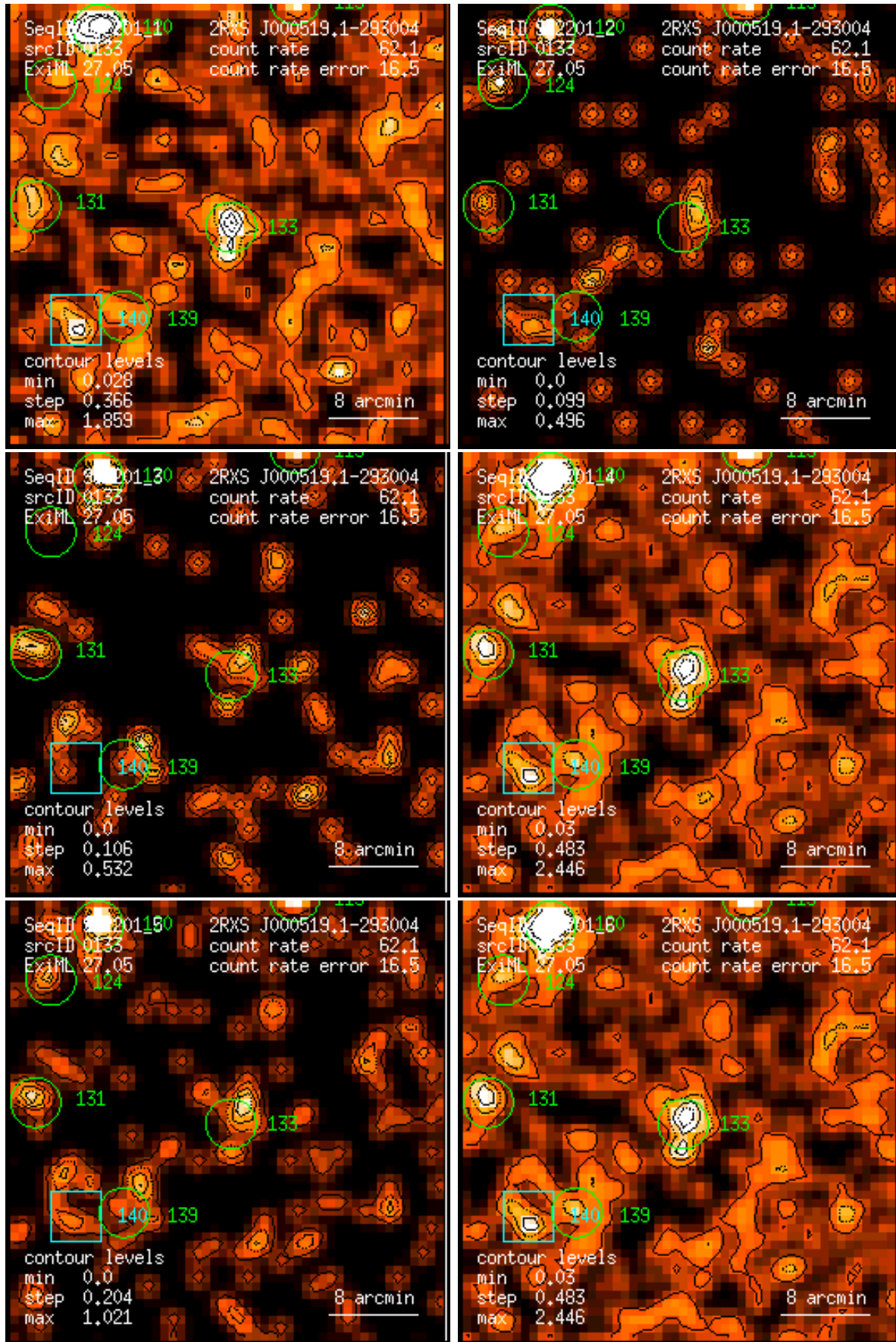
Figure 133: RASS 932201: detection 0133: band rate images, Gaussian filter: (1) PSPC channels 11 – 41, (2) 52 – 90, (3) 91 – 201, (4) 11 – 235, (5) 52 – 201, (6) 11 – 201. Broad band rates in counts/ks. Band rate contour levels in counts/ks/arcmin 2 .
