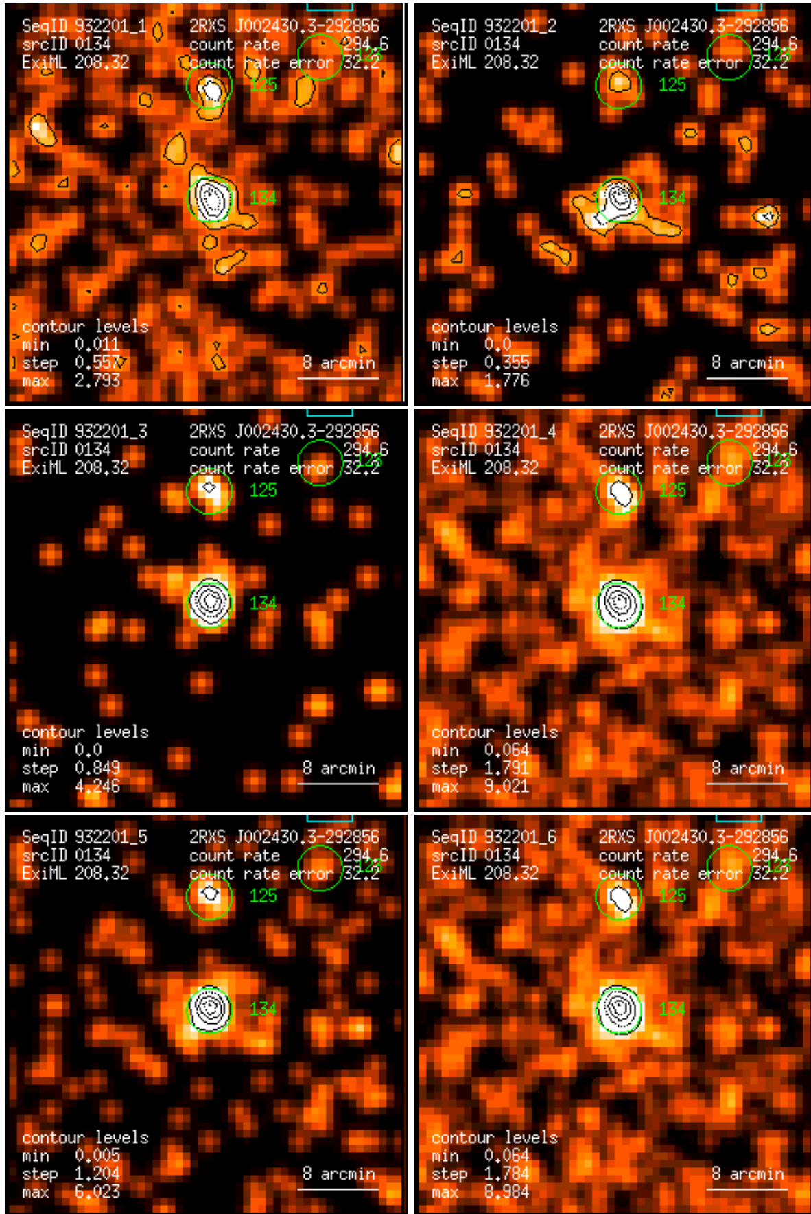
Figure 134: RASS 932201: detection 0134: band rate images, Gaussian filter: (1) PSPC channels 11 – 41, (2) 52 – 90, (3) 91 – 201, (4) 11 – 235, (5) 52 – 201, (6) 11 – 201. Broad band rates in counts/ks. Band rate contour levels in counts/ks/arcmin 2 .
