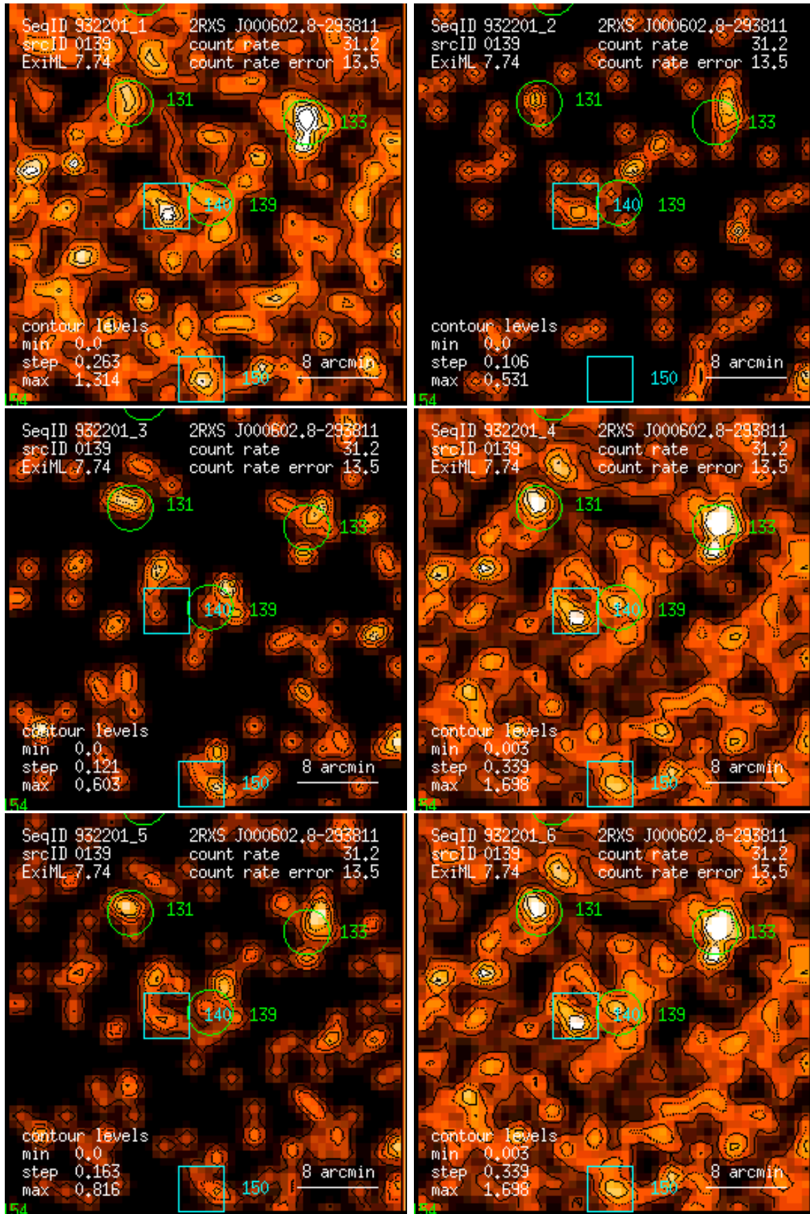
Figure 139: RASS 932201: detection 0139: band rate images, Gaussian filter: (1) PSPC channels 11 – 41, (2) 52 – 90, (3) 91 – 201, (4) 11 – 235, (5) 52 – 201, (6) 11 – 201. Broad band rates in counts/ks. Band rate contour levels in counts/ks/arcmin 2 .
