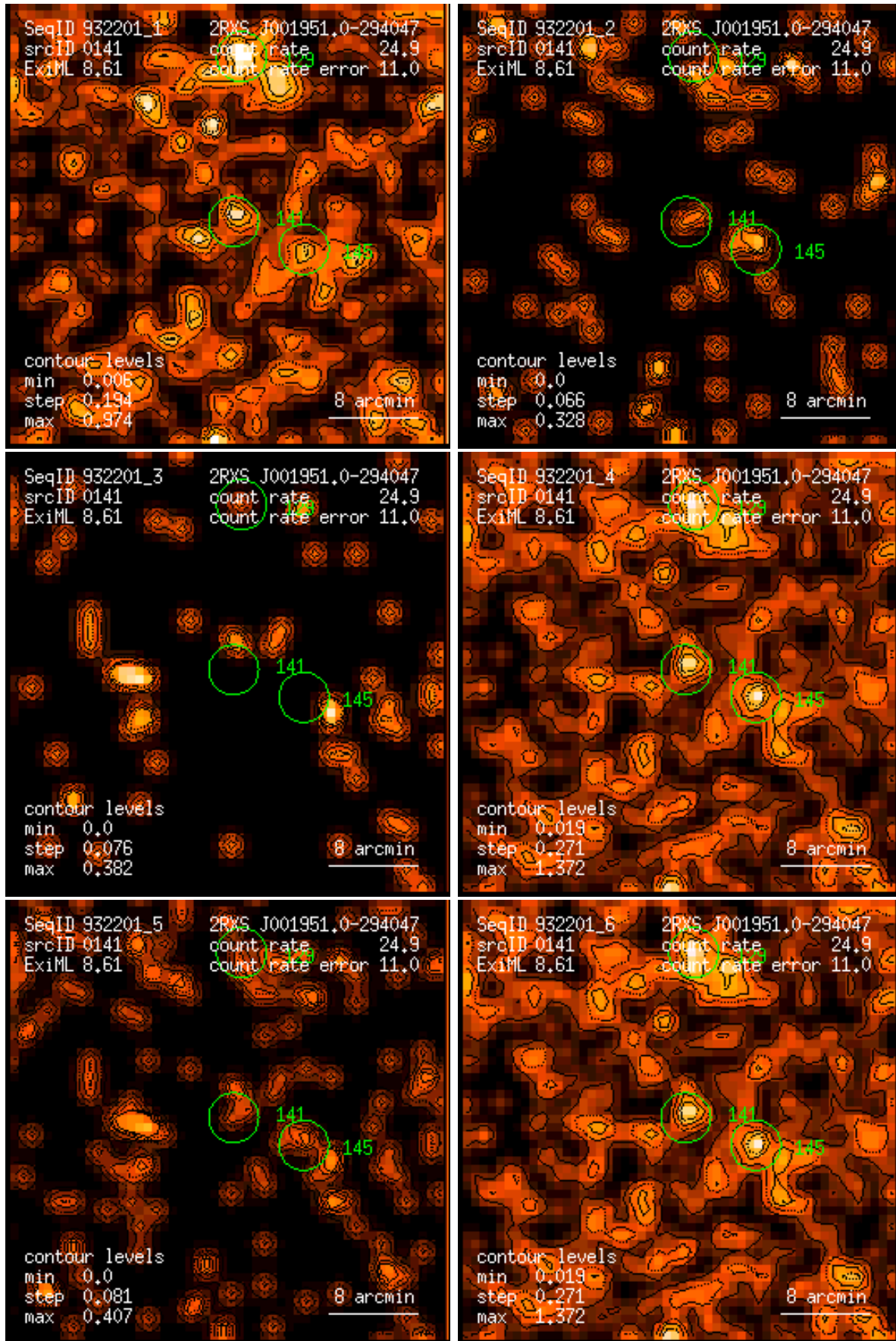
Figure 141: RASS 932201: detection 0141: band rate images, Gaussian filter: (1) PSPC channels 11 – 41, (2) 52 – 90, (3) 91 – 201, (4) 11 – 235, (5) 52 – 201, (6) 11 – 201. Broad band rates in counts/ks. Band rate contour levels in counts/ks/arcmin 2 .
