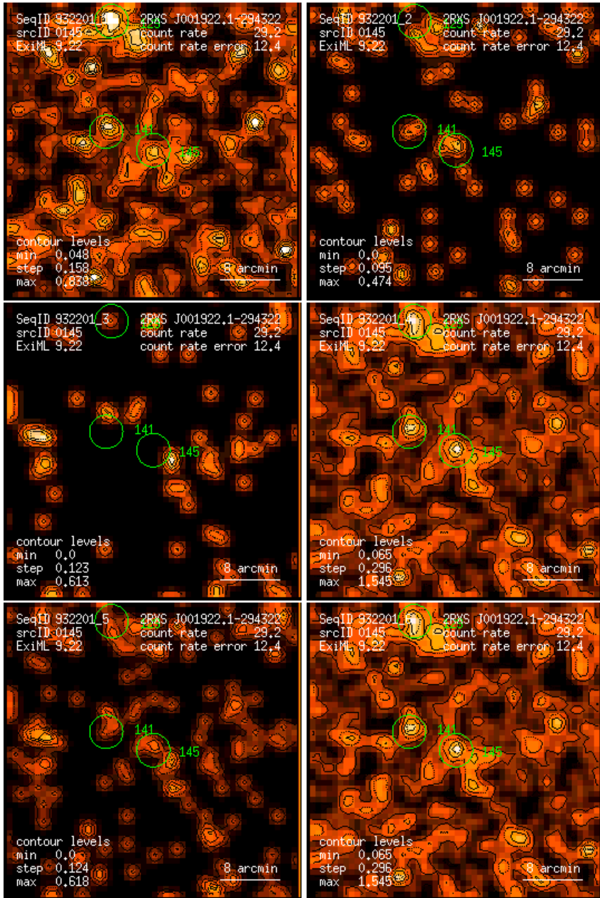
Figure 145: RASS 932201: detection 0145: band rate images, Gaussian filter: (1) PSPC channels 11 – 41, (2) 52 – 90, (3) 91 – 201, (4) 11 – 235, (5) 52 – 201, (6) 11 – 201. Broad band rates in counts/ks. Band rate contour levels in counts/ks/arcmin 2 .
