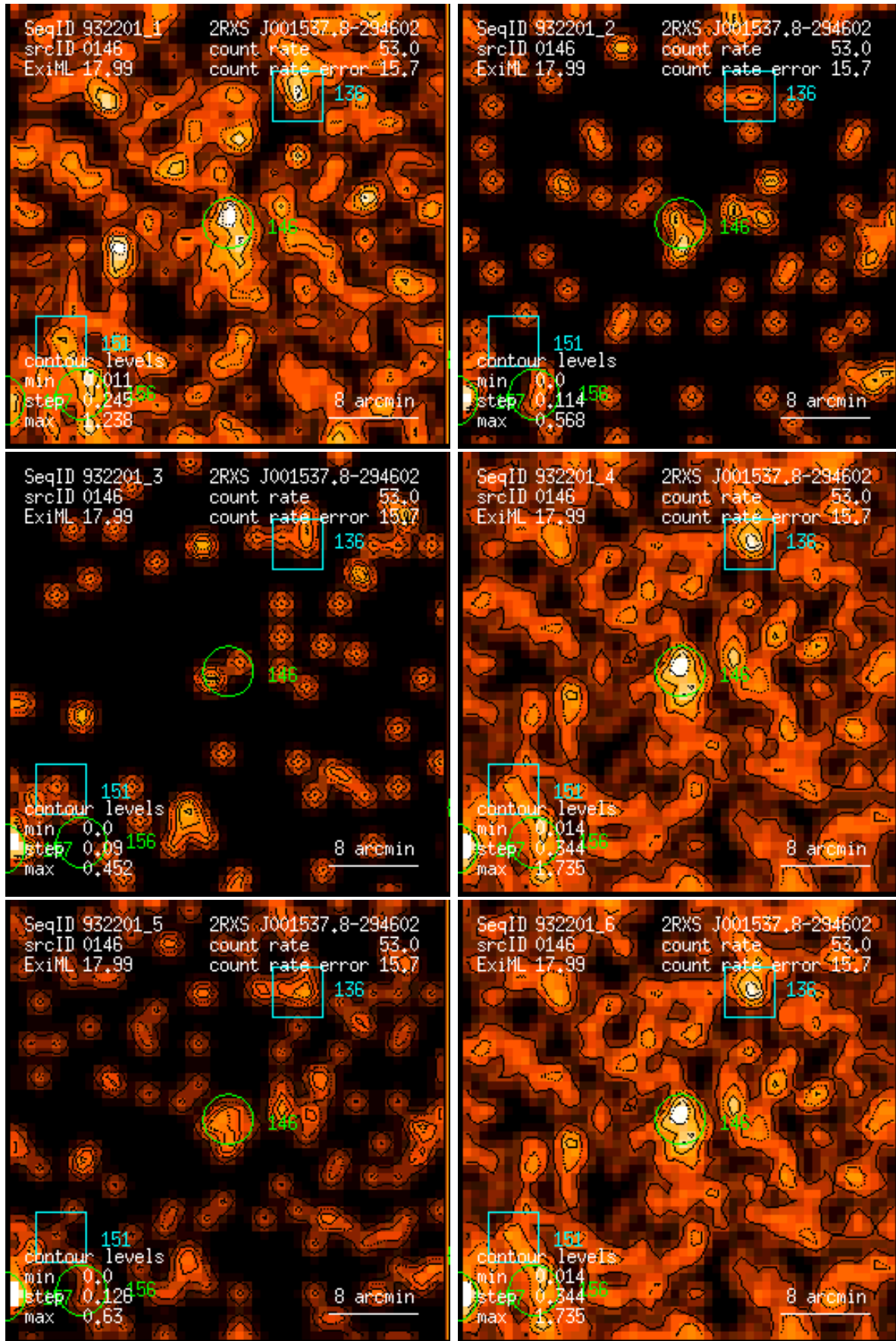
Figure 146: RASS 932201: detection 0146: band rate images, Gaussian filter: (1) PSPC channels 11 – 41, (2) 52 – 90, (3) 91 – 201, (4) 11 – 235, (5) 52 – 201, (6) 11 – 201. Broad band rates in counts/ks. Band rate contour levels in counts/ks/arcmin 2 .
