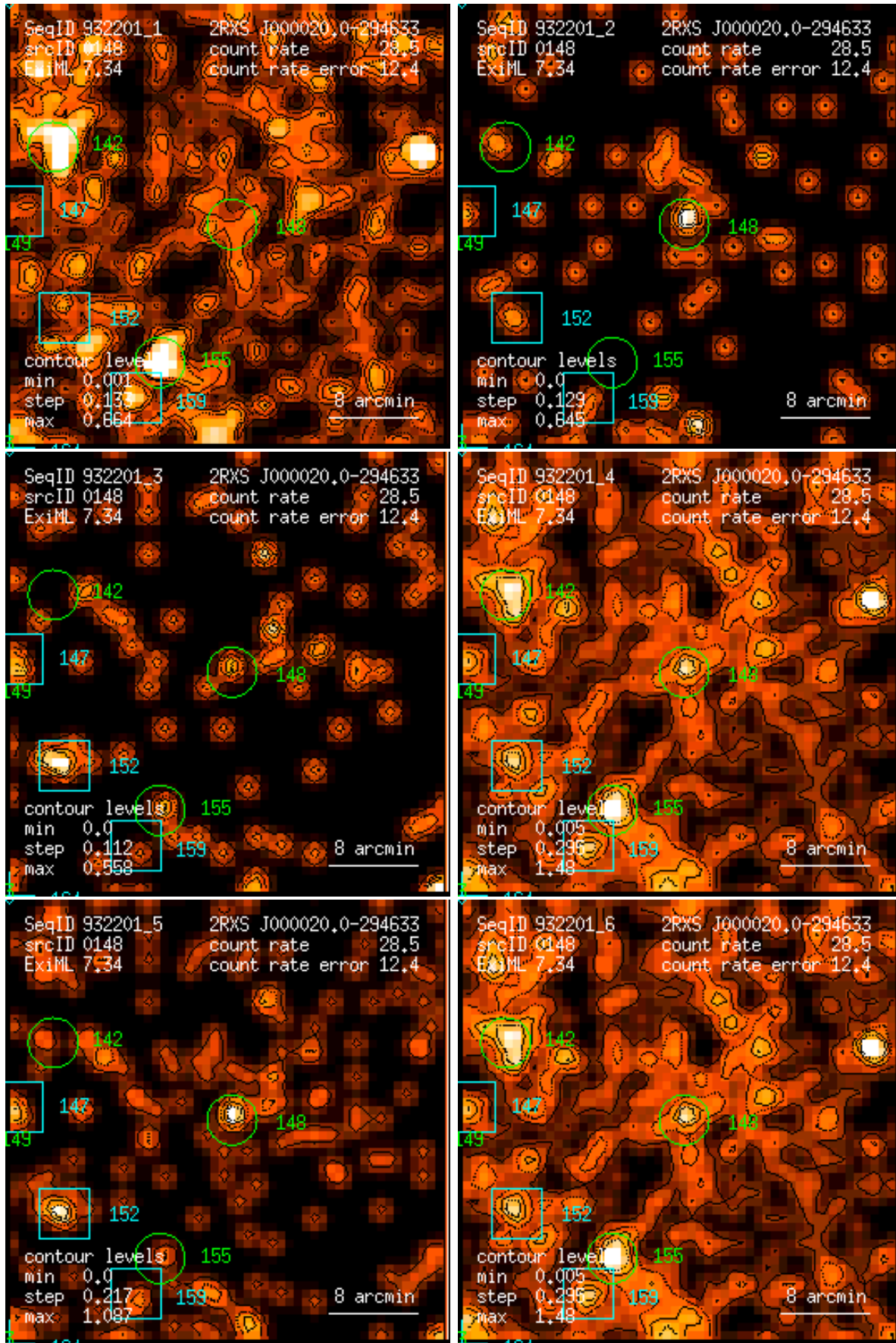
Figure 148: RASS 932201: detection 0148: band rate images, Gaussian filter: (1) PSPC channels 11 – 41, (2) 52 – 90, (3) 91 – 201, (4) 11 – 235, (5) 52 – 201, (6) 11 – 201. Broad band rates in counts/ks. Band rate contour levels in counts/ks/arcmin 2 .
